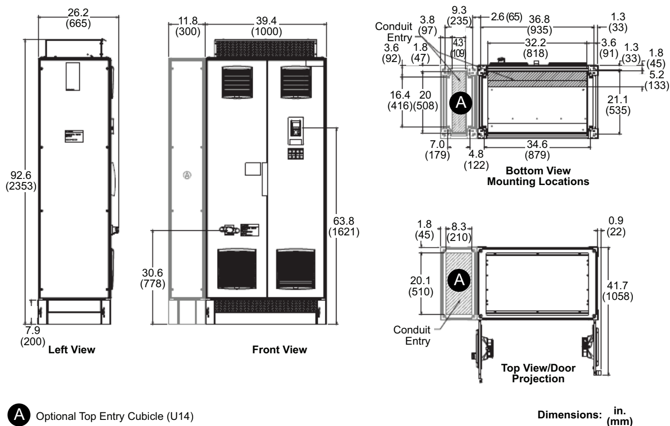
Figure 19 - Conduit Entry and Weights, 300–500 hp ND and 250–400 hp HD @ 460 V, Types 1 and 12
