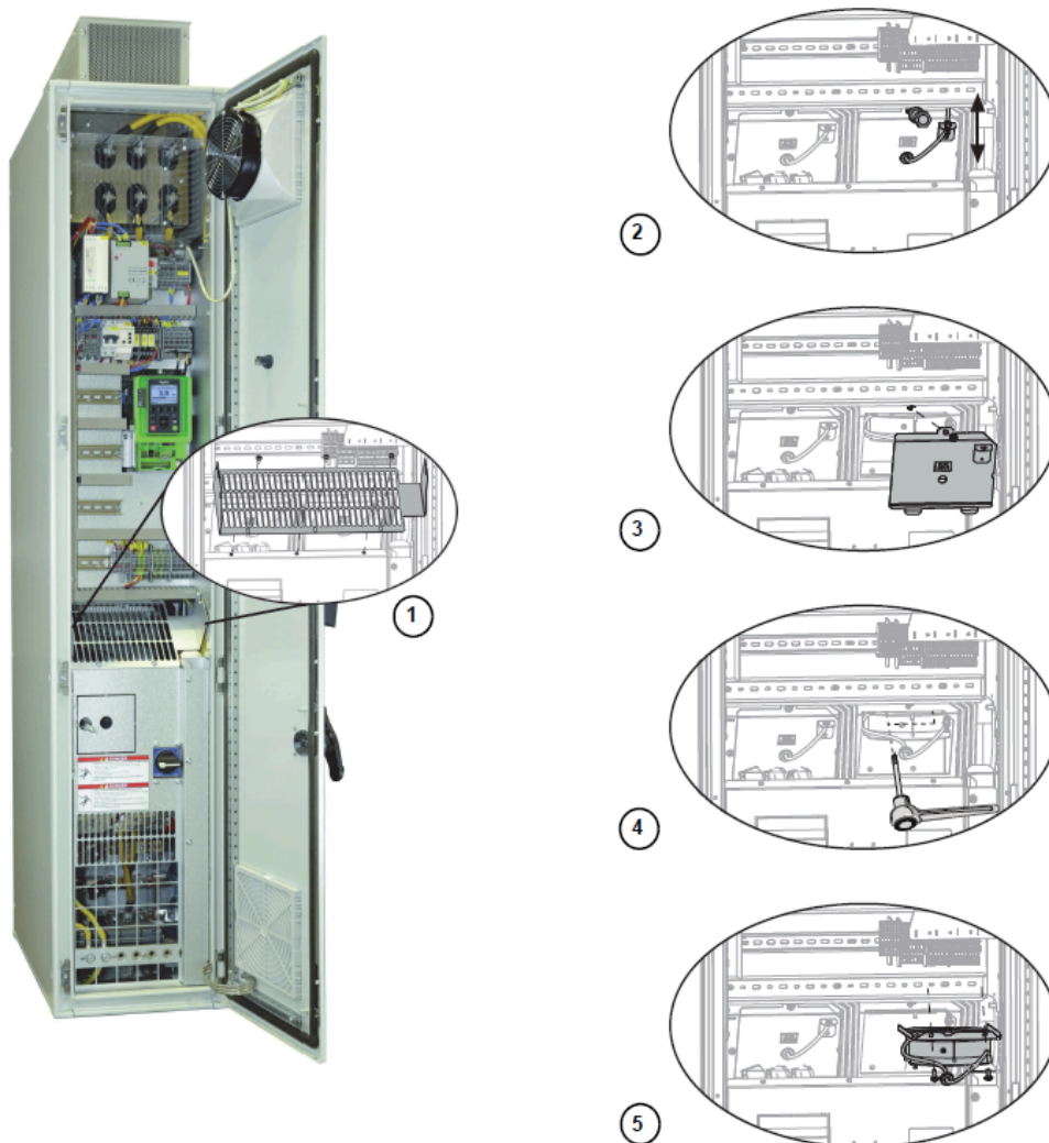
Figure 32 - Installing the Power Fan
