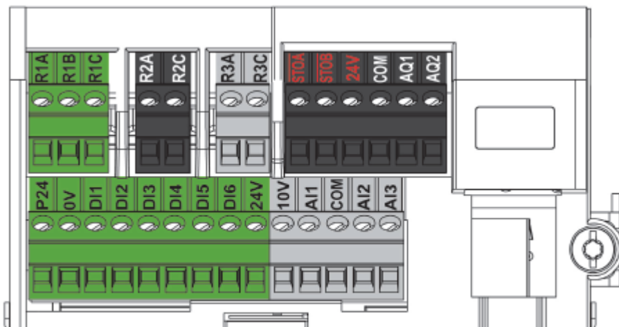
Figure 8 - Control Terminals
