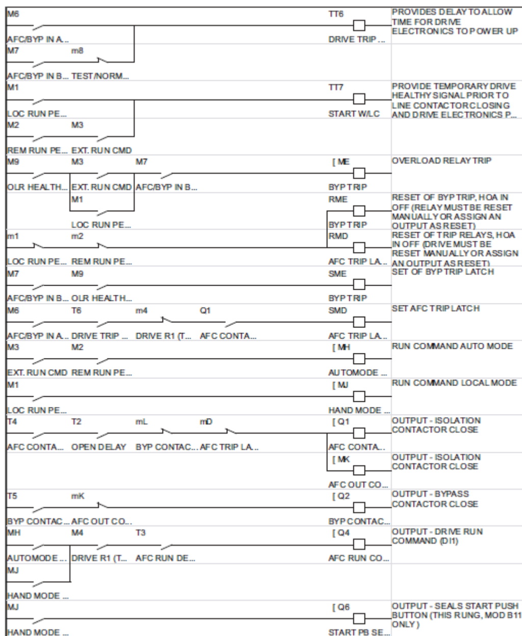
Figure 34 - Zelio Smart Relay Program (continued)
