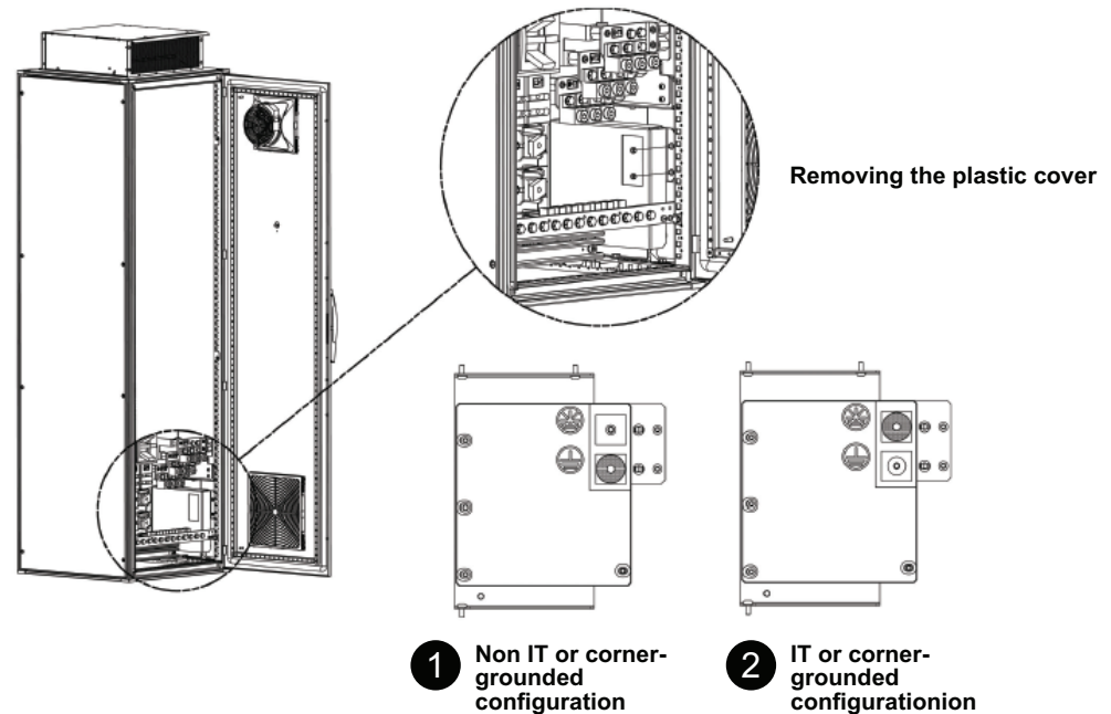
Figure 12 - Settings for 125–700 hp HD, 150–900 hp ND, 460 V Enclosed Drives
