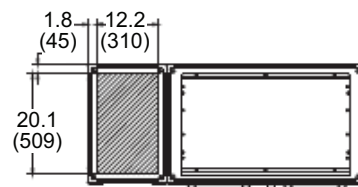
Top View, Front of Unit
