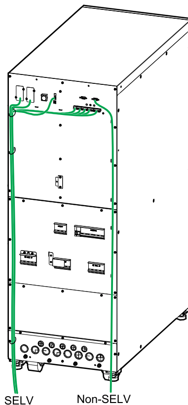
SELV and Non-SELV Cable Routing for 30 - 40 kVA UPS
