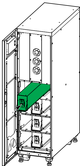
Front View of the 10-20 kVA UPS with One Battery String
