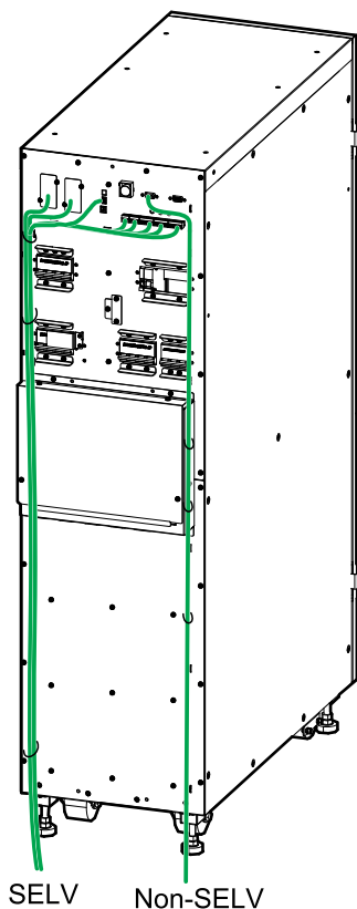
SELV and Non-SELV Cable Routing for 10 - 20 kVA UPS
