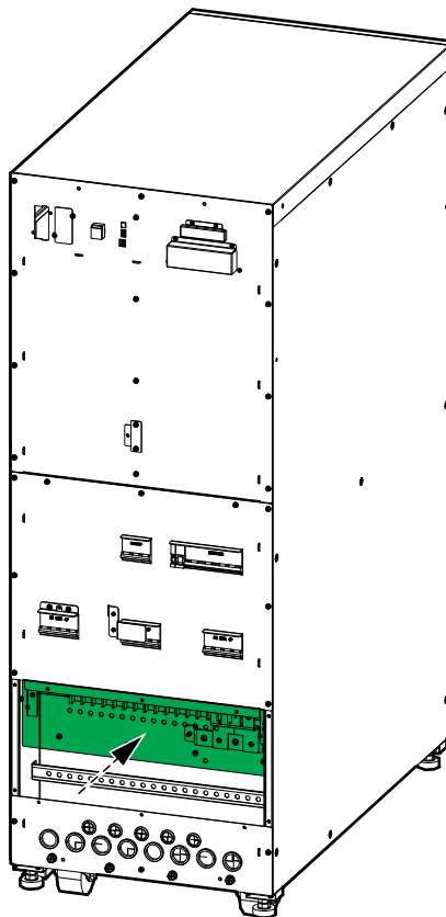
Rear View
