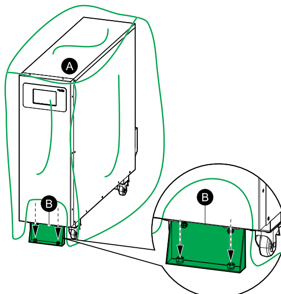
30-40 kVA UPS
