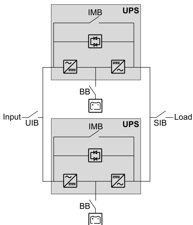
Simplified 1+1 Parallel System – Single Mains
