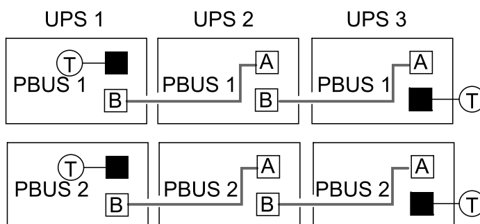
Example of System with Three UPSs in Parallel
