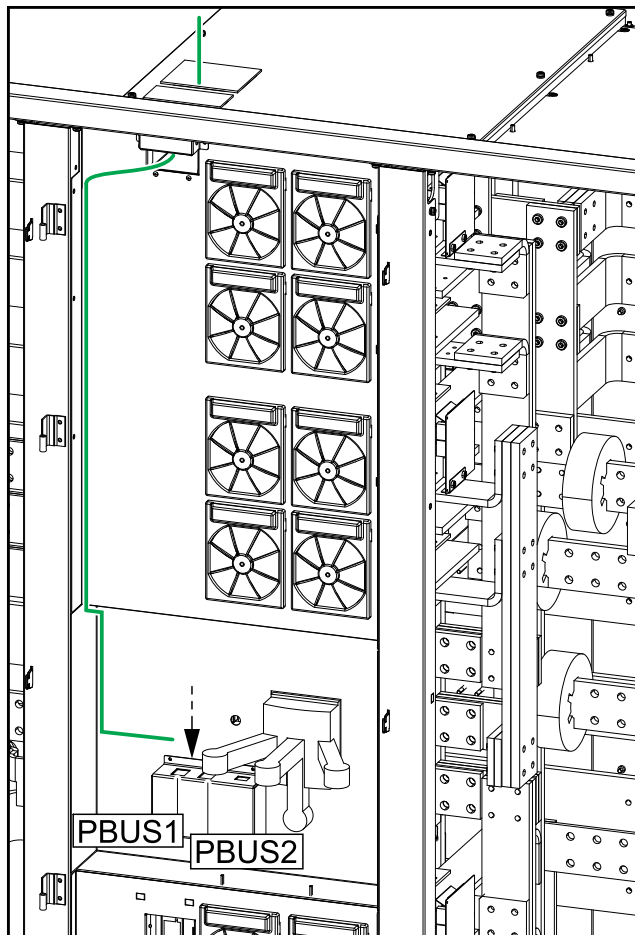
Top Cable Entry Systems
