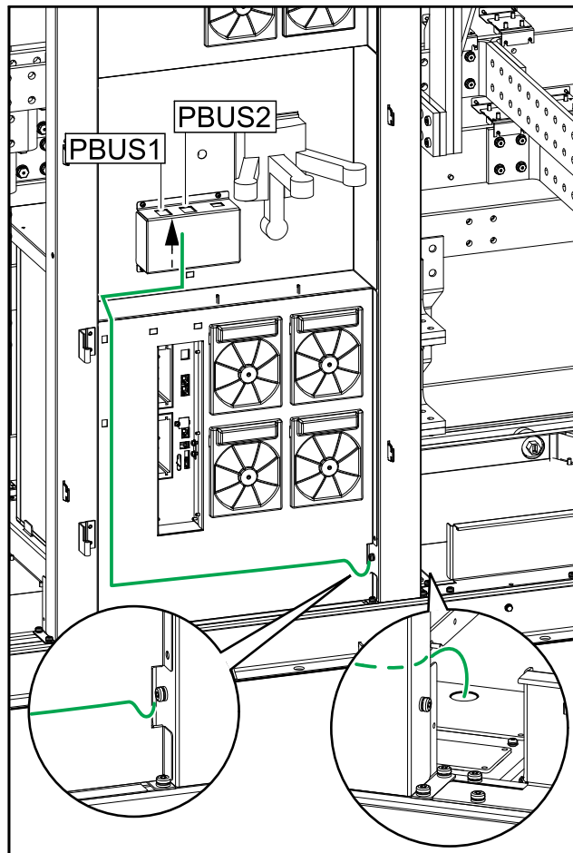
Bottom Cable Entry Systems
