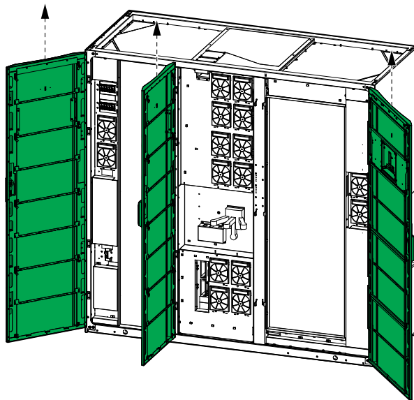
Front View of the Power Cabinet
