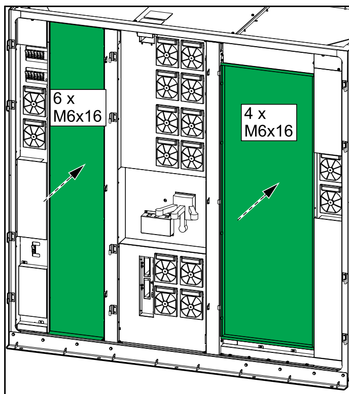
Front View of the I/O Cabinet
