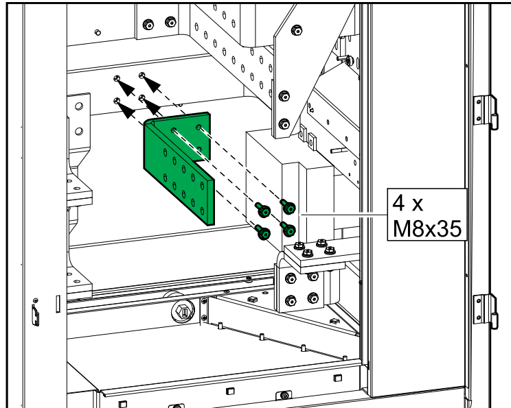
Front View of the I/O Cabinet
