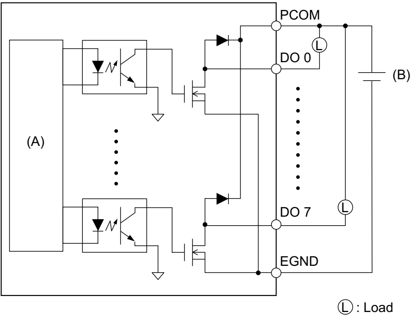
(A) Internal circuit (B) 24 Vdc
