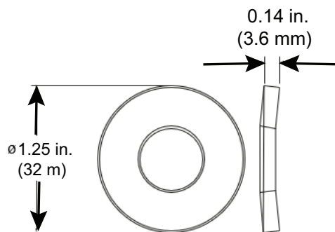
Figure 20 - Belleville Washer
