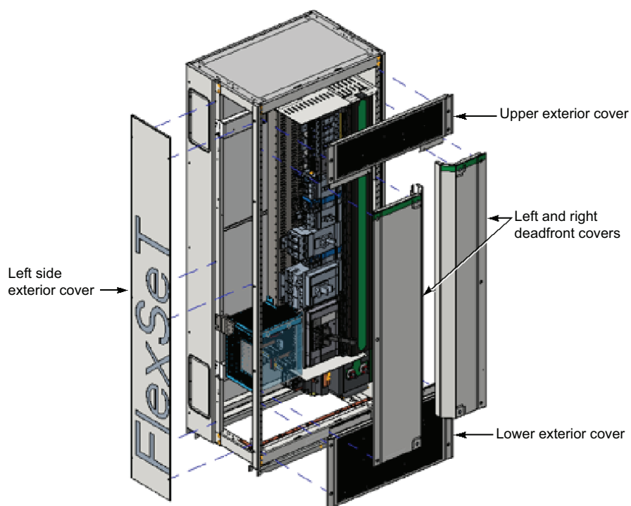
Figure 53 - Removing Covers
