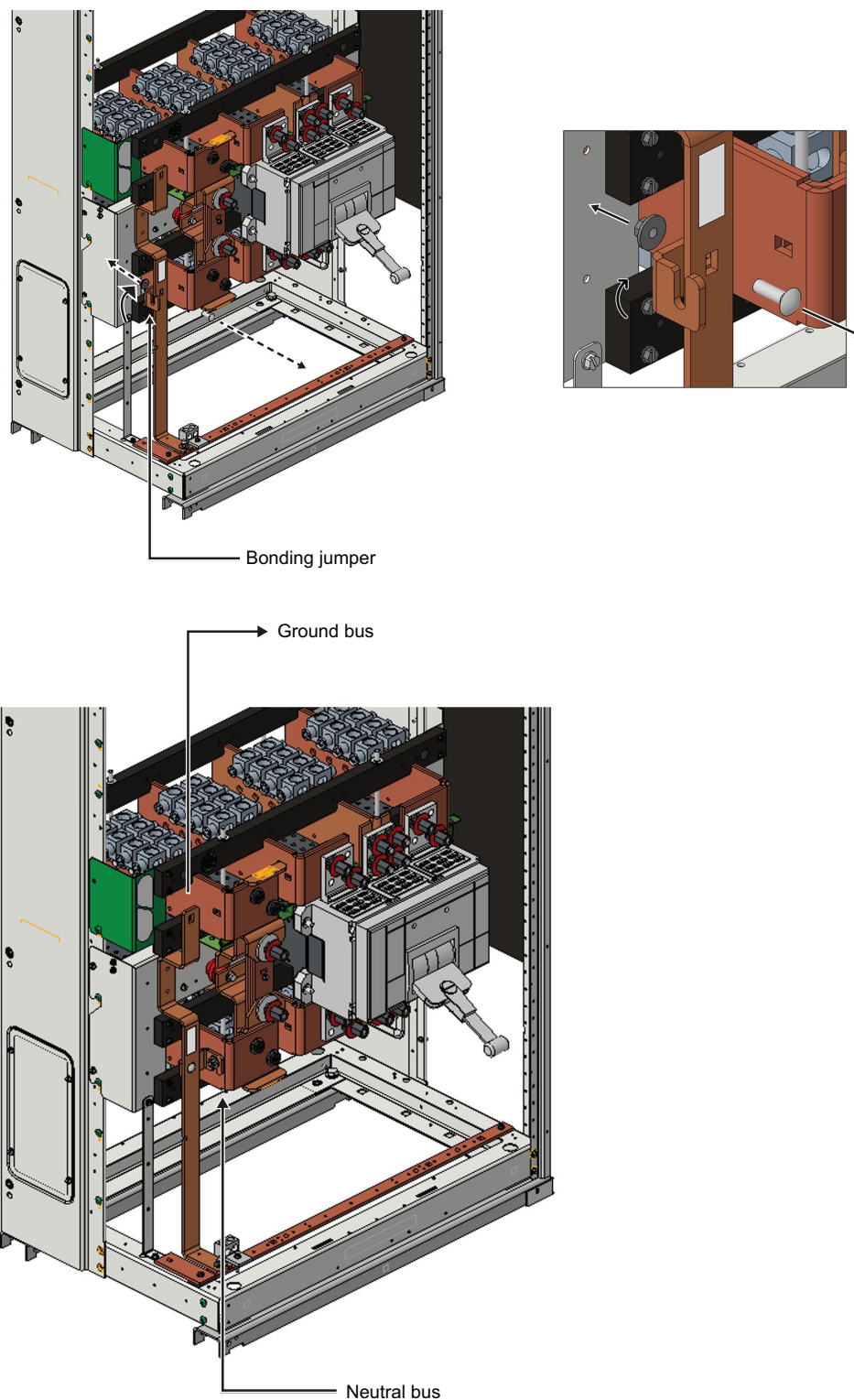
Figure 48 - Bonding Jumper Connection at Lug-in Lug-out Main (Bottom Feed)
