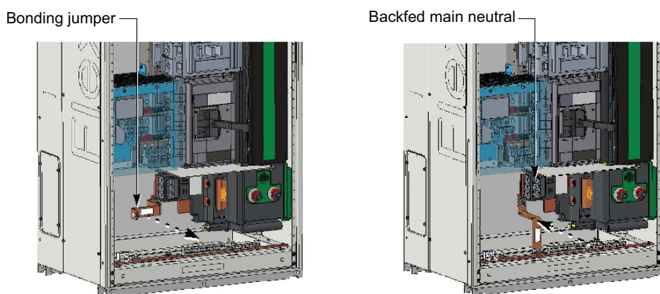
Figure 45 - Bonding Jumper Connection at Backfed Neutral
