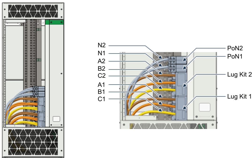
Figure 60 - 3P4W Wiring Example With Plug on Neutrals (PoN)
