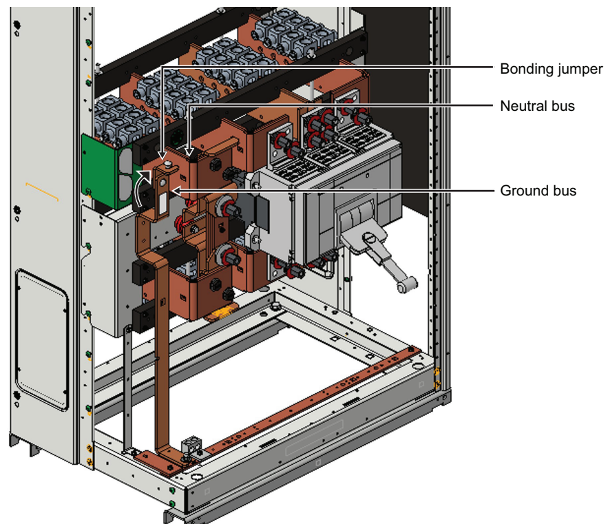
Figure 47 - Bonding Jumper Connection at Lug-in Lug-out Main (Top Feed)
