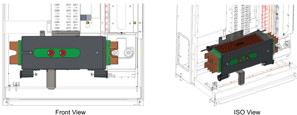
Figure 28 - Completed Bridge Assembly in the I-Line Section
