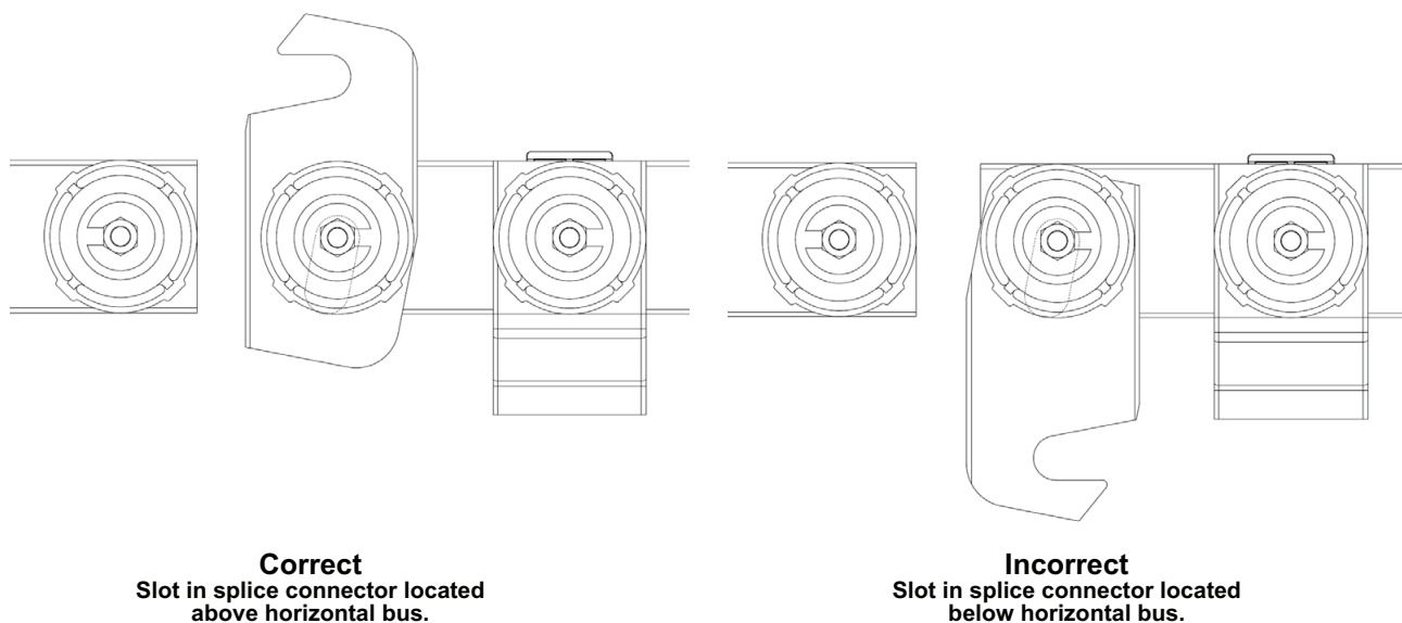
Figure 37 - Proper Orientation of Splice Connector
