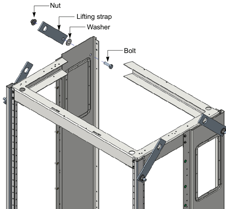
Figure 4 - Hardware Assembly Order in Enclosures With Knockouts in Vertical Corner Channels
