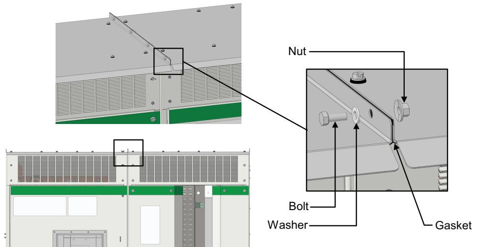
Figure 16 - Joining the Driphoods in NEMA 2 Enclosures
