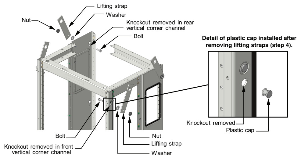
Figure 4 - Hardware Assembly Order in Enclosures With Knockouts in Vertical Corner Channels
