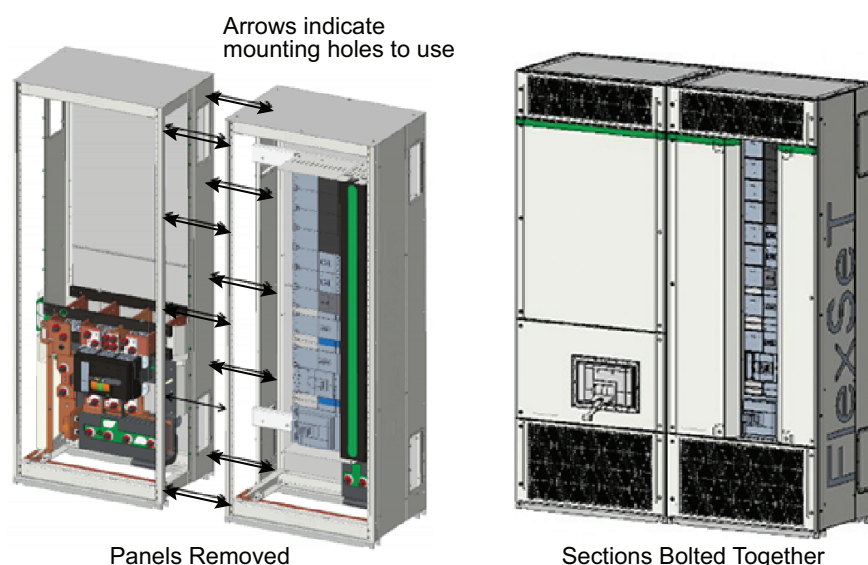
Figure 13 - Joining Indoor Switchboard Sections
