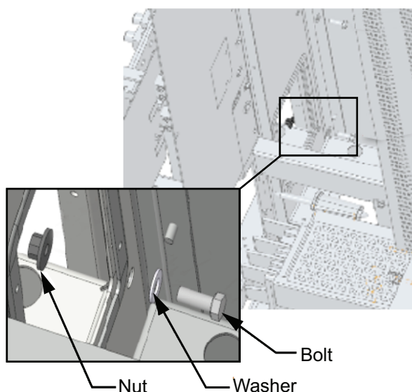
Figure 15 - Hardware Orientation in Enclosures that Include Threaded Inserts on the Rear and Front Vertical Channels
