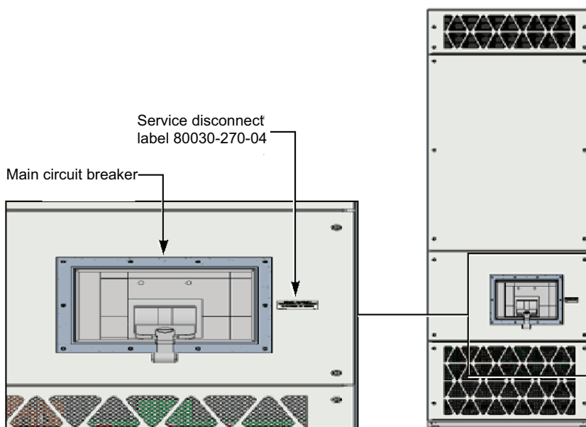
Figure 42 - Label Location on Main Circuit Breaker
