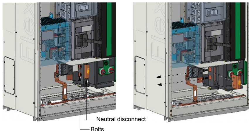
Figure 49 - Removing Neutral Disconnect at Backfed Neutral
