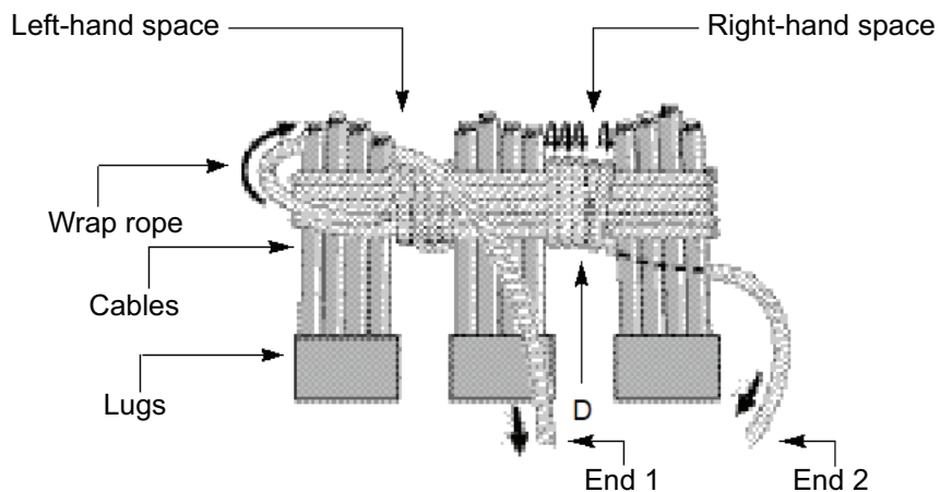
Figure 65 - Finish Wrapping the Space Between Cables
