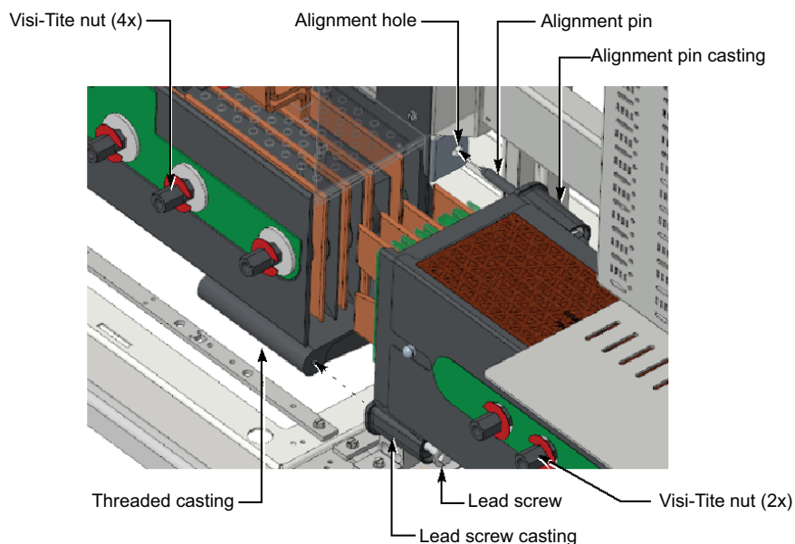
Figure 30 - Connecting Assemblies
