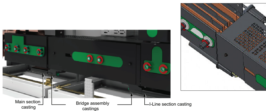
Figure 31 - Fully Connected Bridge Assembly
