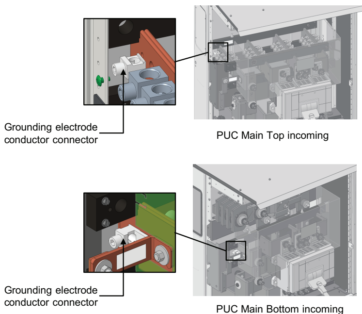
Figure 44 - Grounding Electrode Connector in PUC Main
