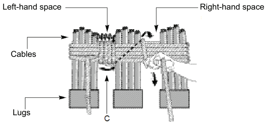
Figure 64 - Wrapping the Space Between Cables
