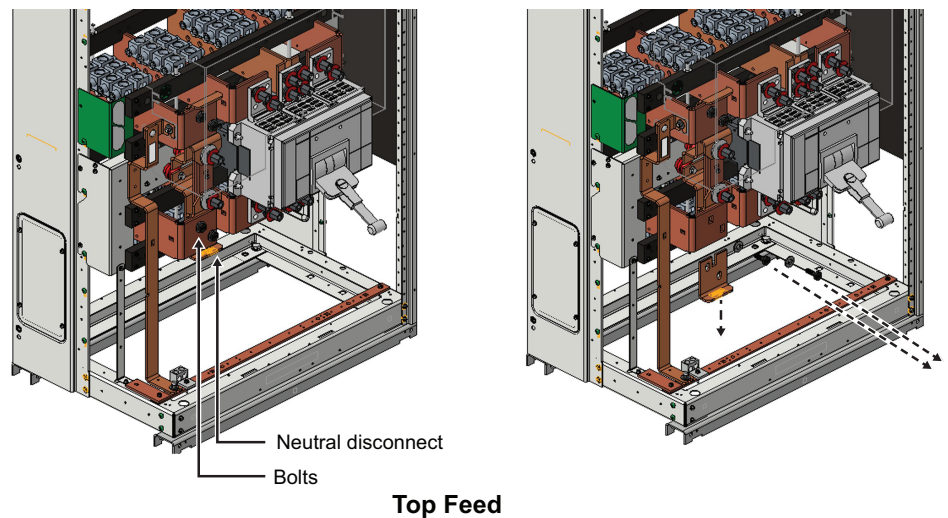
Figure 51 - Removing Neutral Disconnect at Lug-in Lug-out Main (Top Feed)
