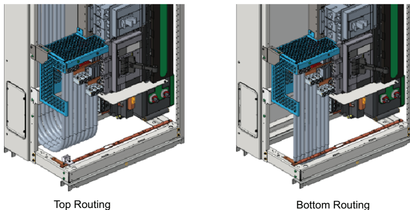
Figure 56 - Routing Cables
