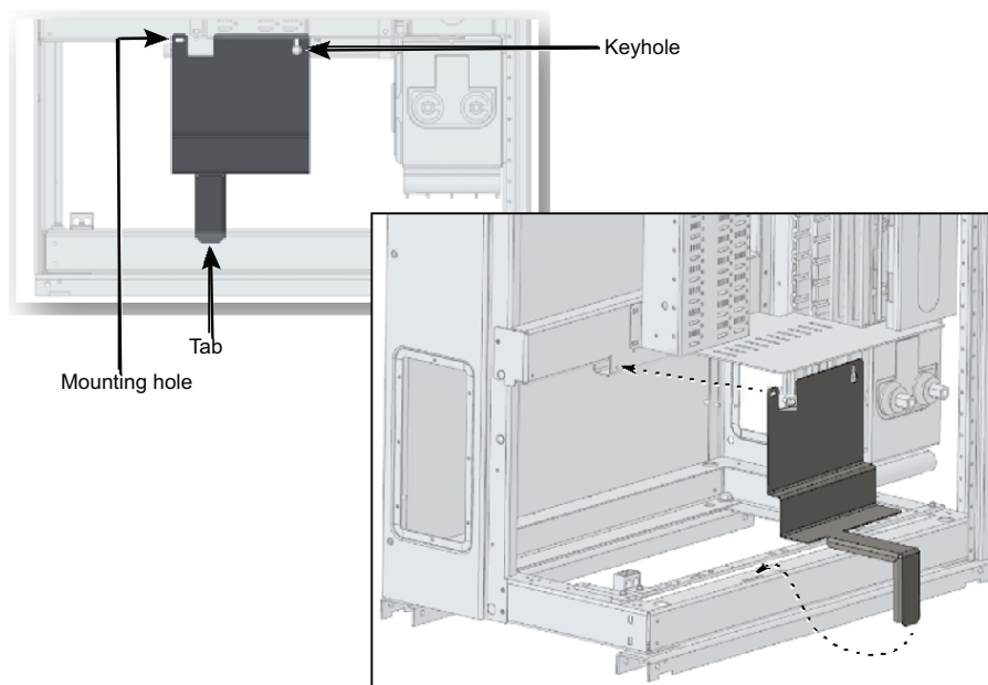
Figure 27 - Bridge Assembly
