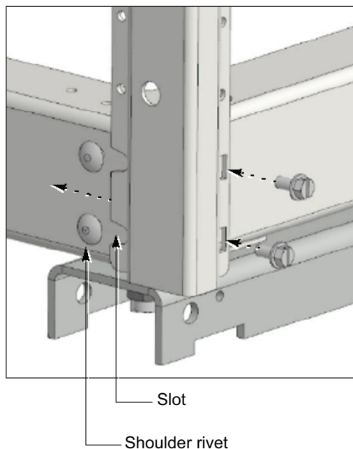
Figure 32 - Installing Front Corner Channels
