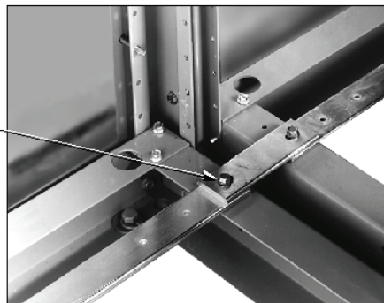
Figure 40 - Ground Bus Splice Connection
