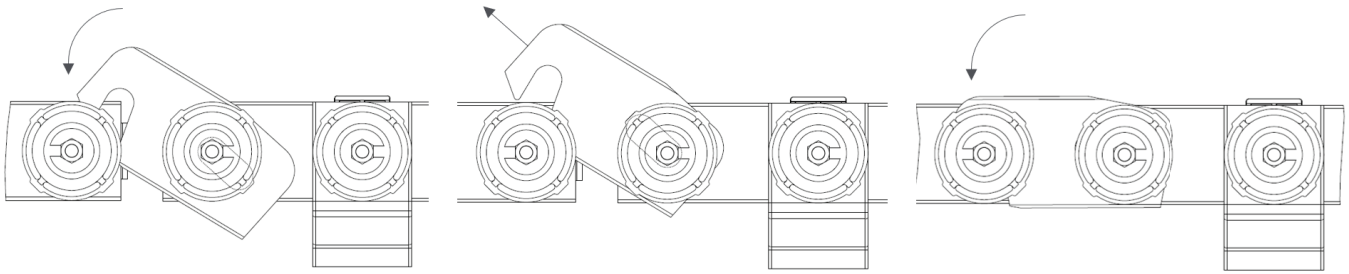
Figure 39 - Installation of Splice Connectors
