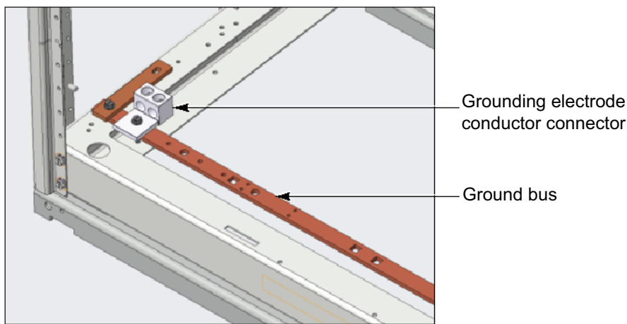
Figure 44 - Grounding Electrode Connector in PUC Main
