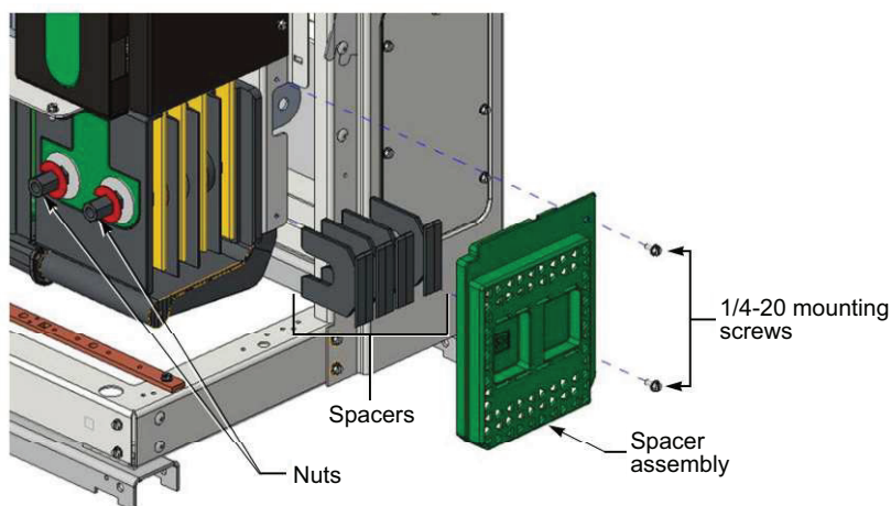
Figure 34 - Remove Spacer Assembly
