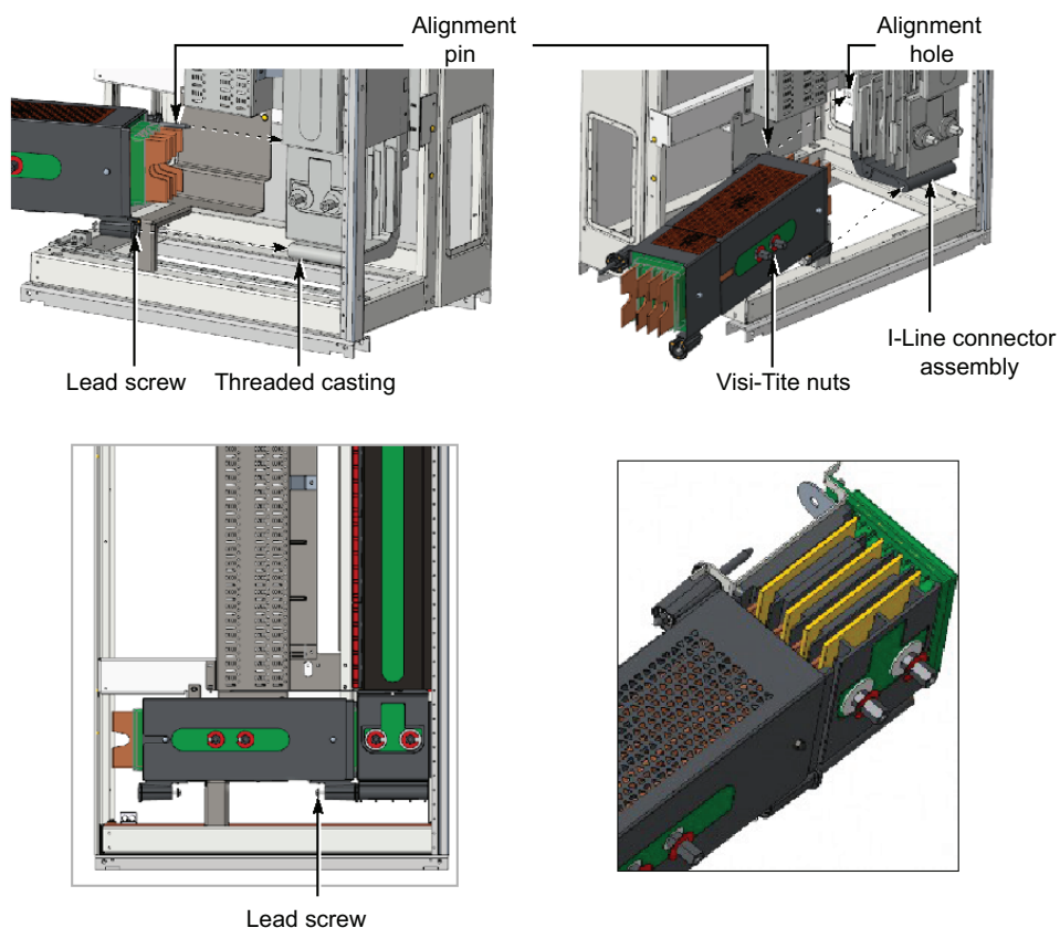
Figure 29 - Bridge Assembly Installation
