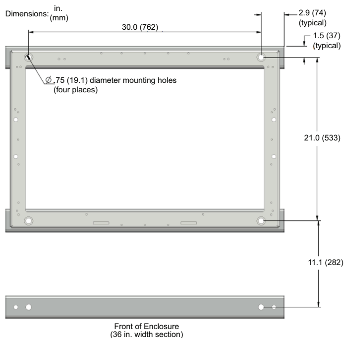
Figure 18 - Outdoor Switchboard Base Channel Floor Anchor Bolt Locations
