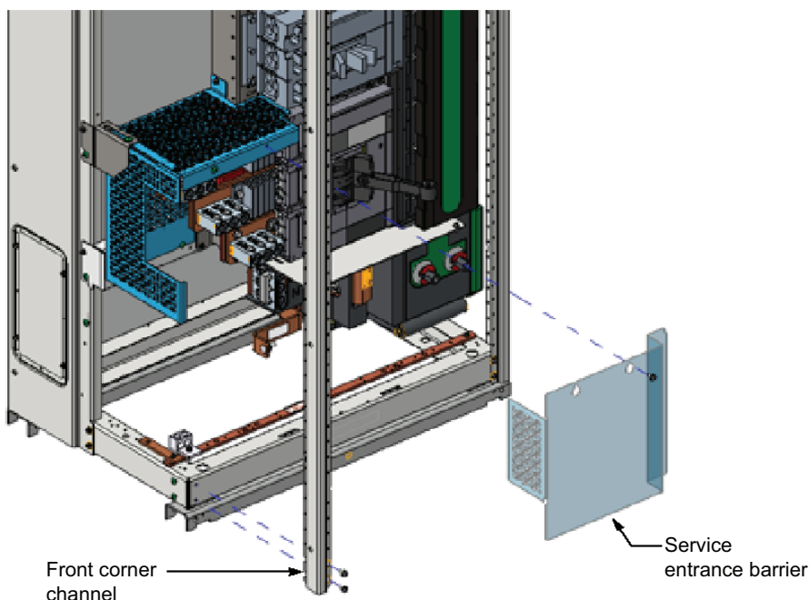
Figure 54 - Removing Front Corner Channel and Barrier
