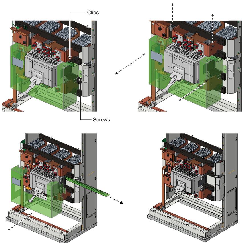
Figure 26 - Barrier Removal for Lug-in Lug-out Main Bottom Incoming
