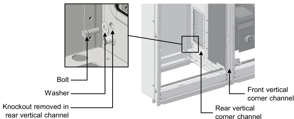
Figure 15 - Hardware Orientation in Enclosures that Include Threaded Inserts on the Rear and Front Vertical Channels
