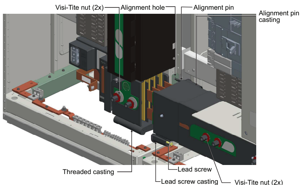
Figure 35 - Bridge Installation to I-Line Stack with Neutral Assembly
