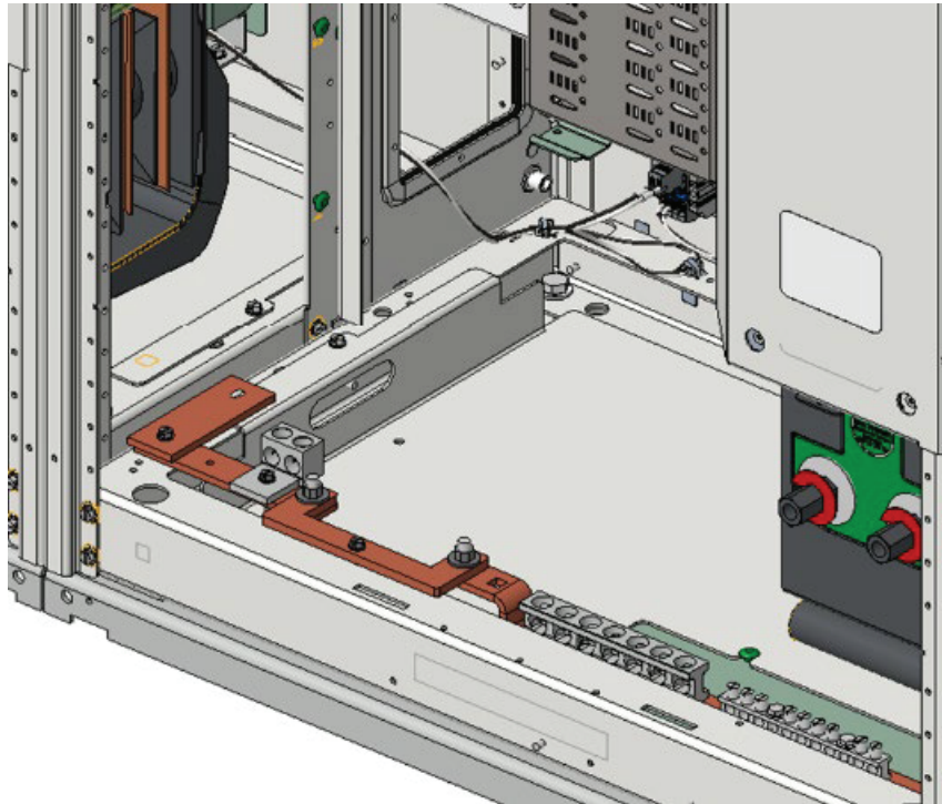
Figure 58 - Connecting Heater Extension Harness
