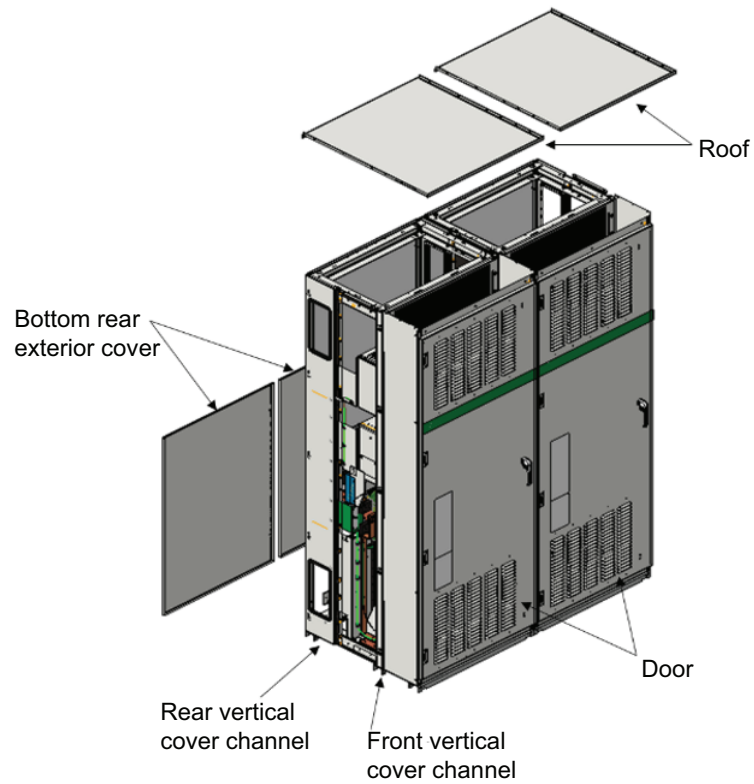
Figure 11 - Parts with Gaskets in NEMA 2, PUC Main
