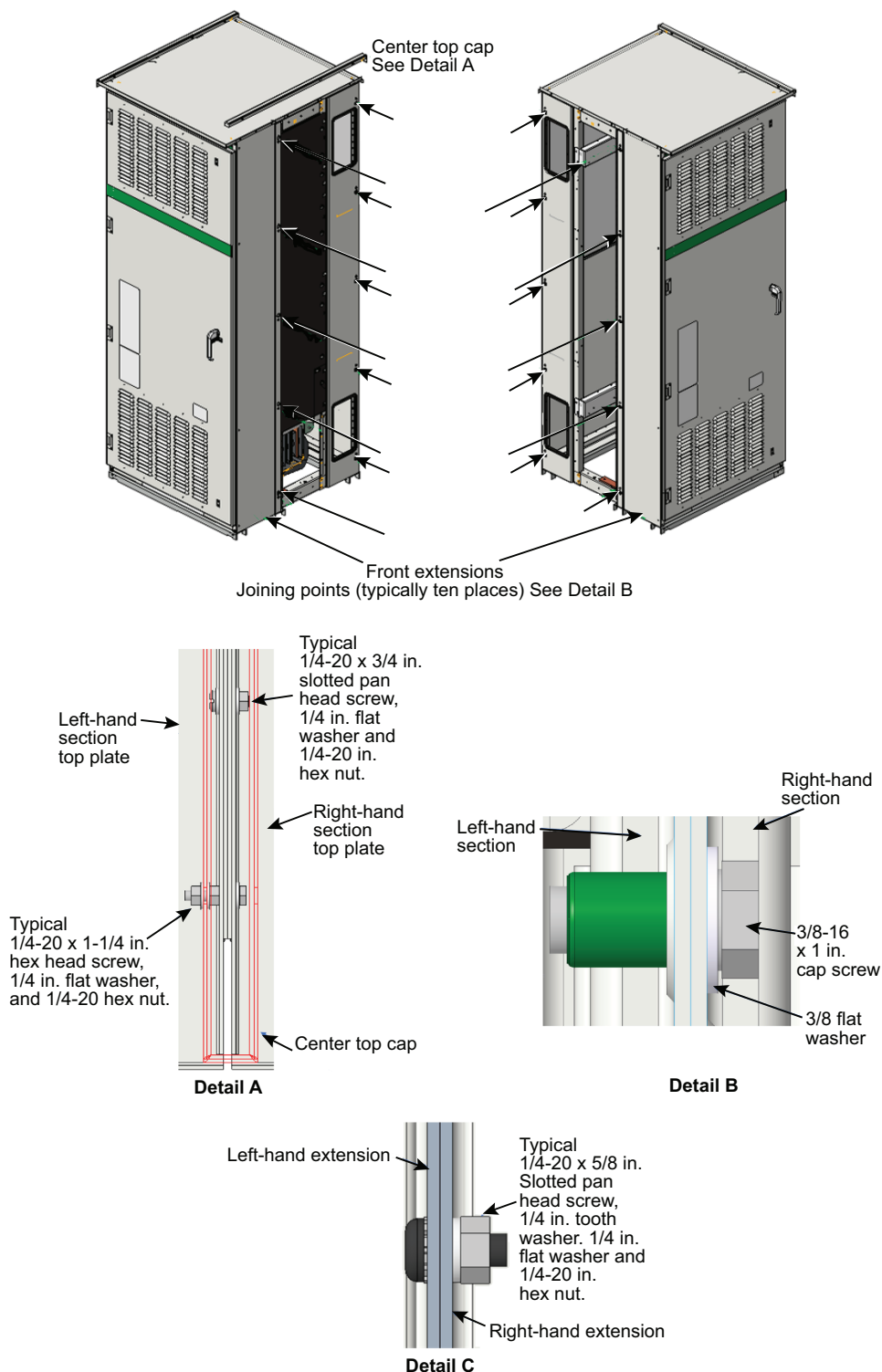
Figure 7 - Joining Shipping Sections—Outdoor Switchboards
