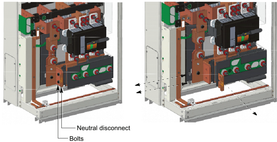
Figure 50 - Removing Neutral Disconnect Main
