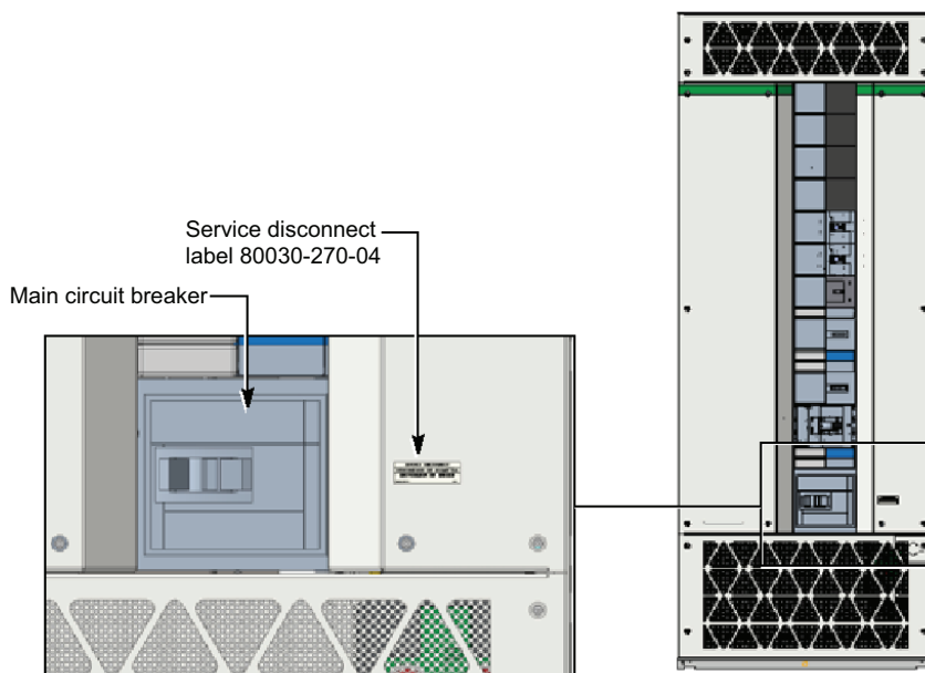
Figure 41 - Label Location on I-Line
