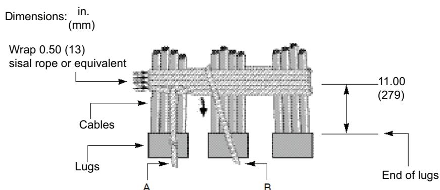
Figure 63 - Wrapping Cables (neutral cables not shown)
