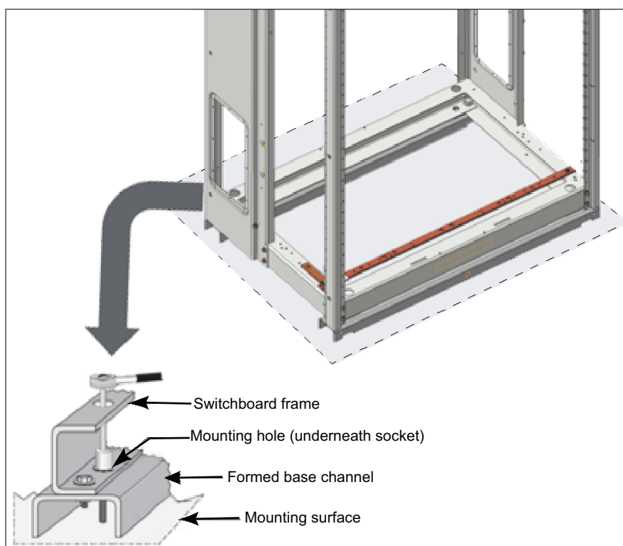
Figure 21 - Anchoring Detail
