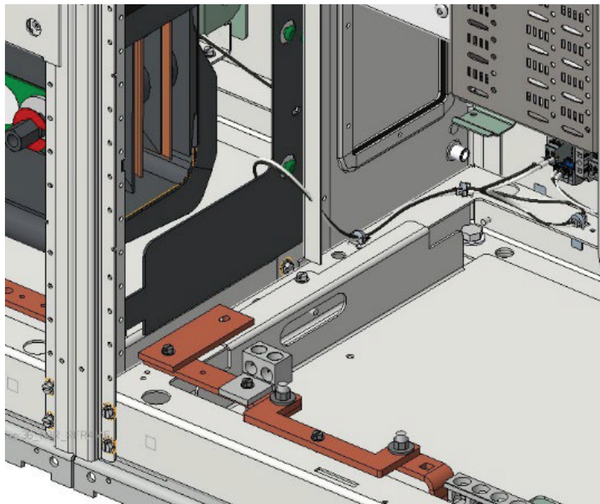
Figure 59 - Connecting Heater Extension Harness When Service Entrance Barrier is Provided
