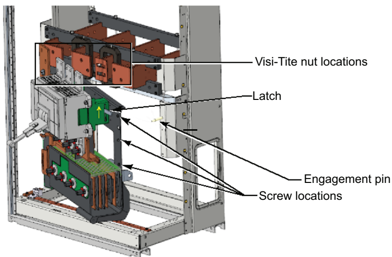
Figure 24 - Rotating Bus Assembly
