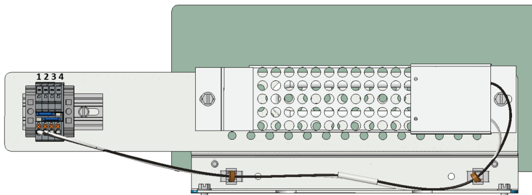
Figure 57 - Terminal Block Identification
