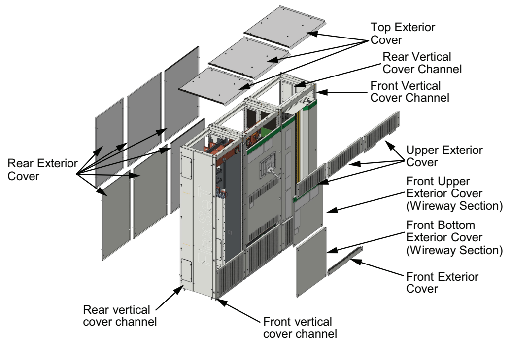
Figure 11 - Parts with Gaskets in NEMA 2, PUC Main
