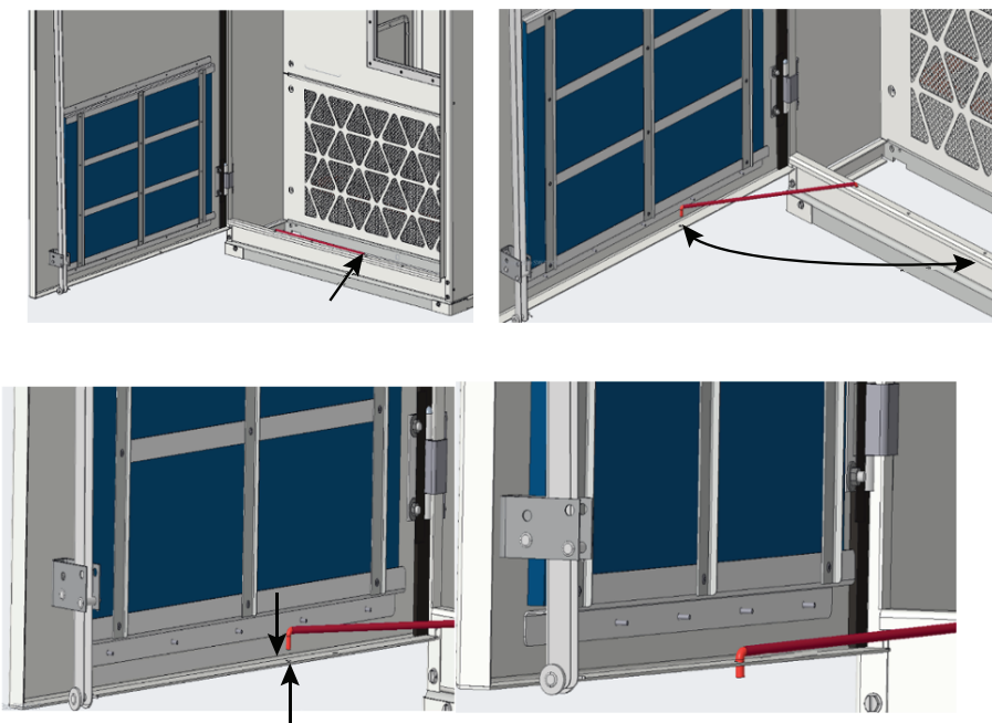
Figure 9 - Doorstop Insertion
