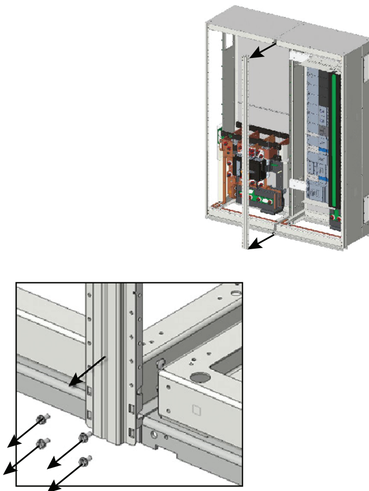
Figure 22 - Channel Removal
