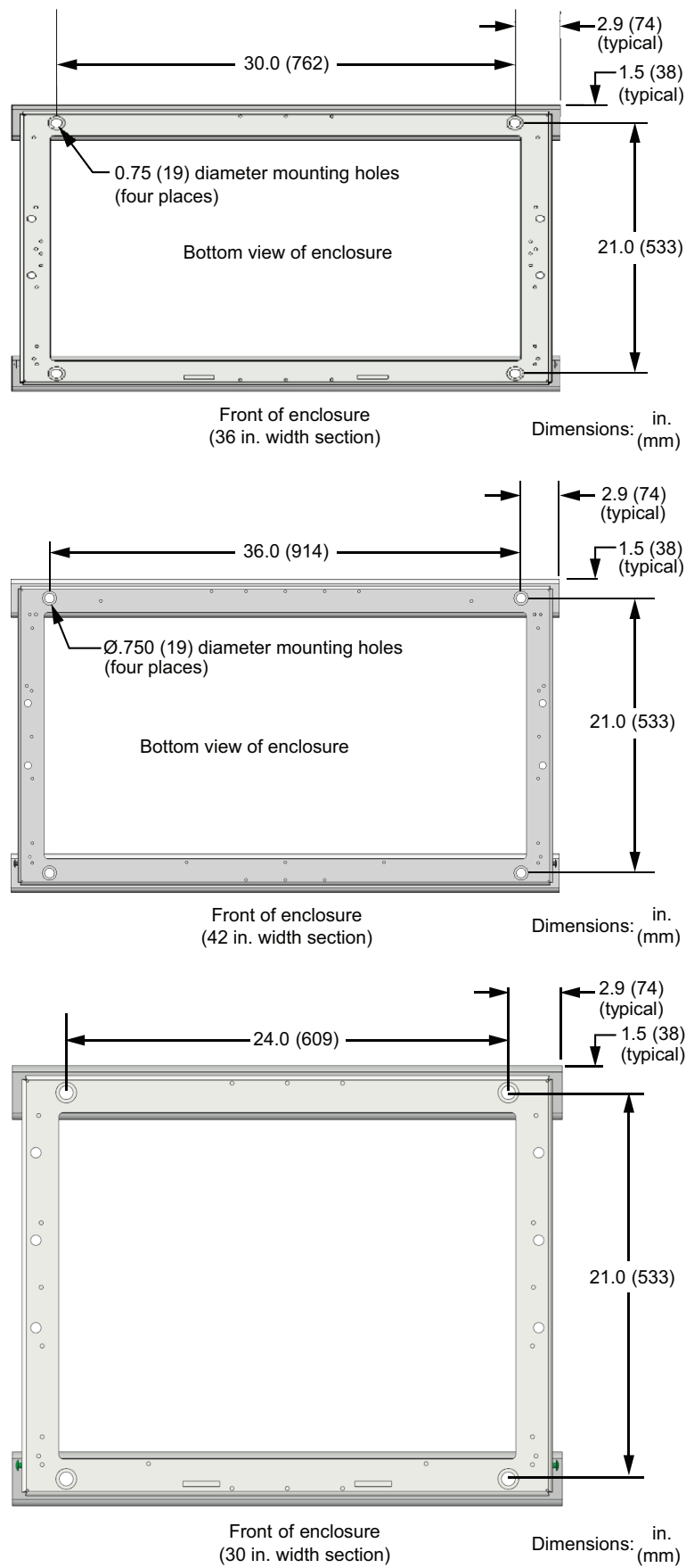
Figure 17 - Base Channel Floor Anchor Bolt Locations
