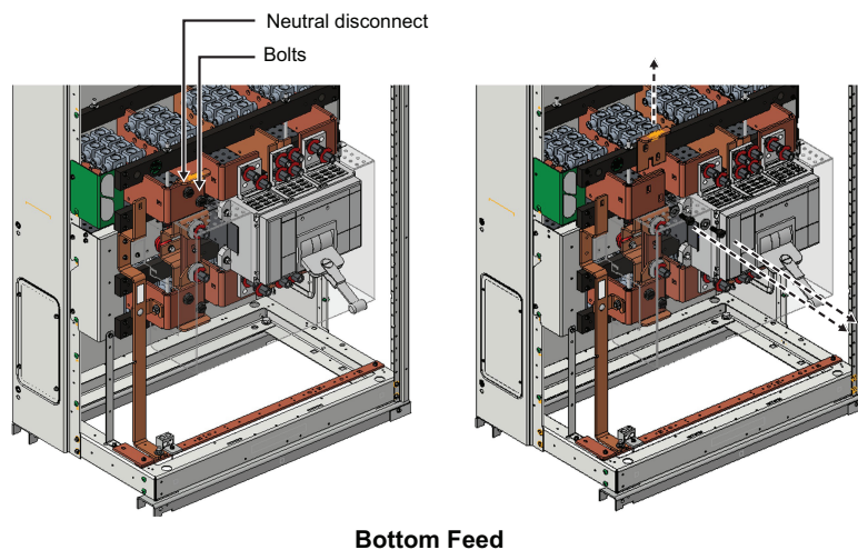
Figure 52 - Removing Neutral Disconnect at Lug-in Lug-out Main (Bottom Feed)
