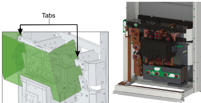
Figure 23 - Barrier Removal
