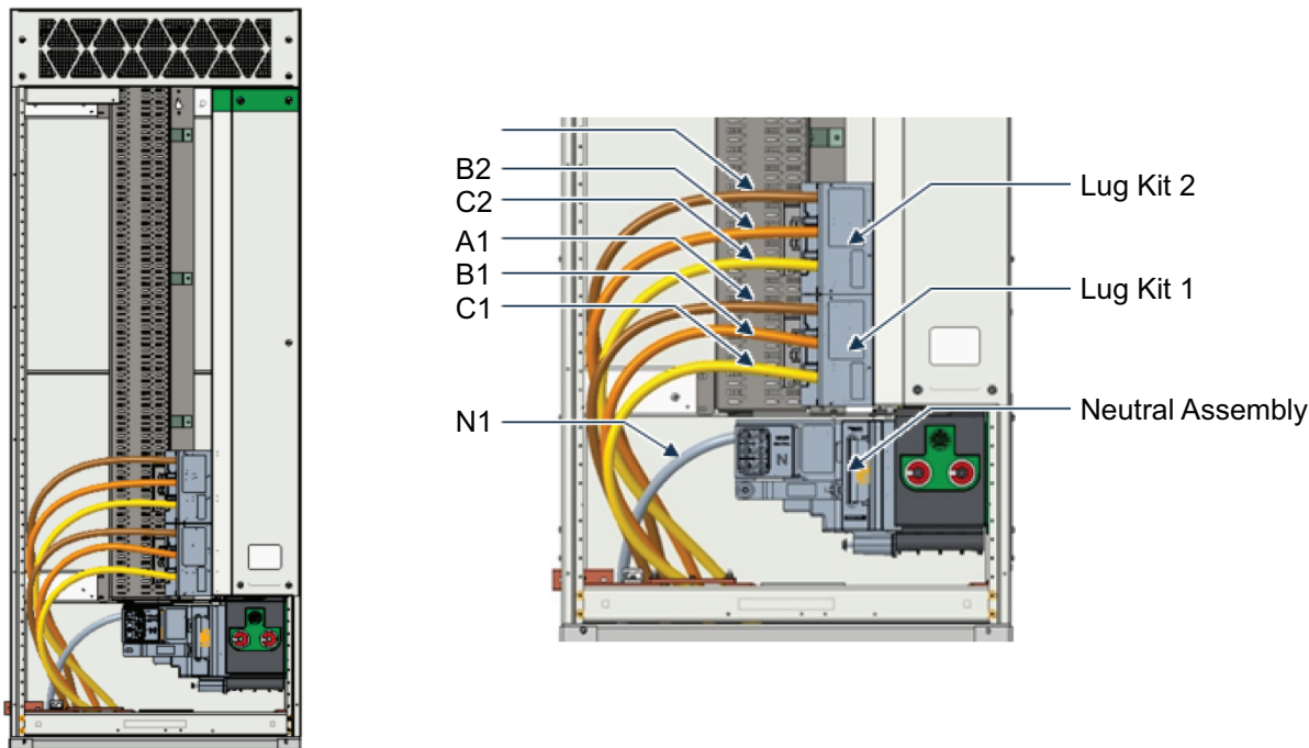
Figure 61 - 3P4W Wiring Example With Neutral Assembly
