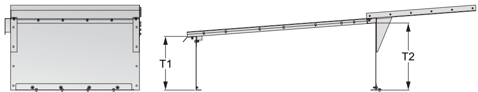
Figure 5 Dimension of External Exhaust 24 kV
