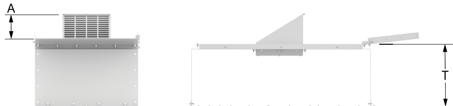
Figure 3 Dimension of Internal Exhaust
