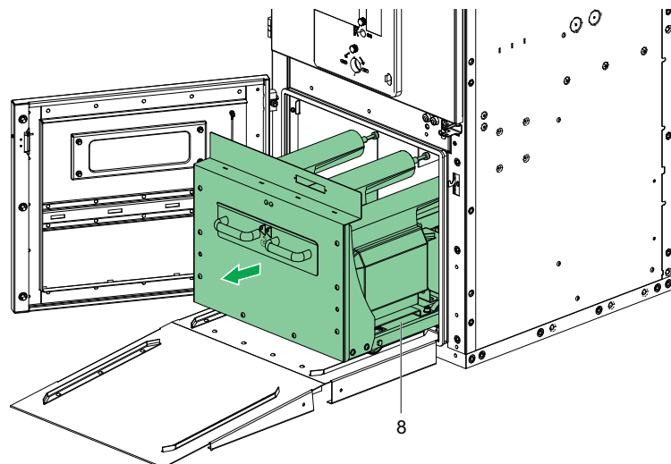
Figure 61 Position the Withdrawable VT
