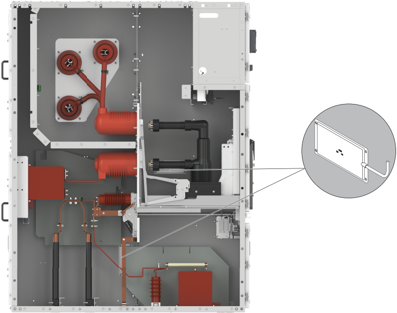
Figure 15 Location of Heater in MCSeT Switchgear
