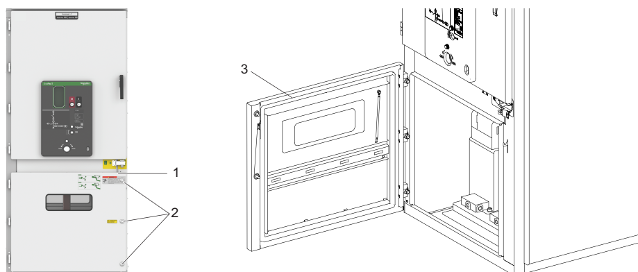
Figure 54 Access to Cable Compartment
