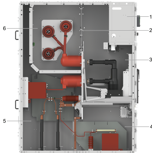
Figure 53 Access to the Main Circuit Compartments of I/F Cubicle
