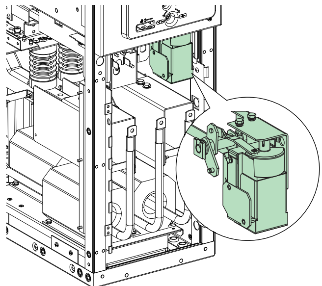
Figure 25 Feeder with Contactor Cubicle Cable Compartment Door interlock
