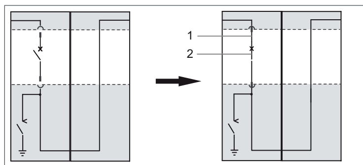
Figure 51 Coupling Busbar Sections via BSC and EvoPacT HVX Trucks
