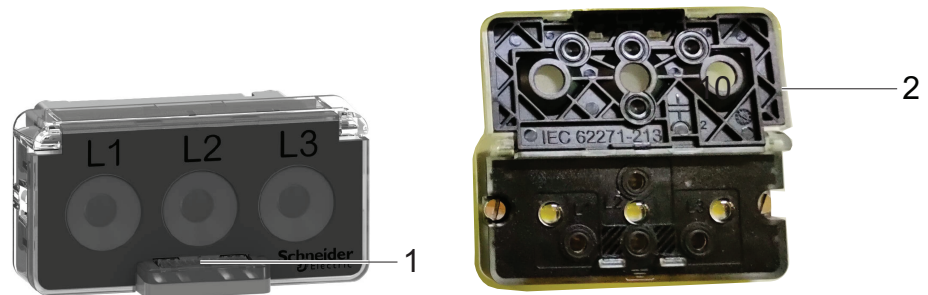
Figure 16 VDIS
