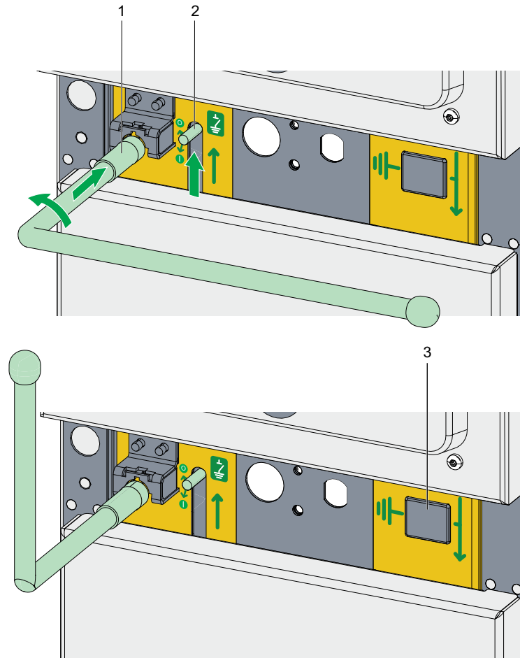
Figure 48 Switching E/S OFF
