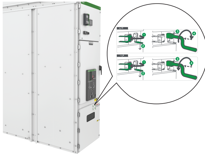
Figure 10 Label of E/S Manual Operating Instructions
