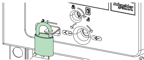
Figure 32 Padlock on Truck - Manual Insertion of Contactor Truck Blocked by Padlock
