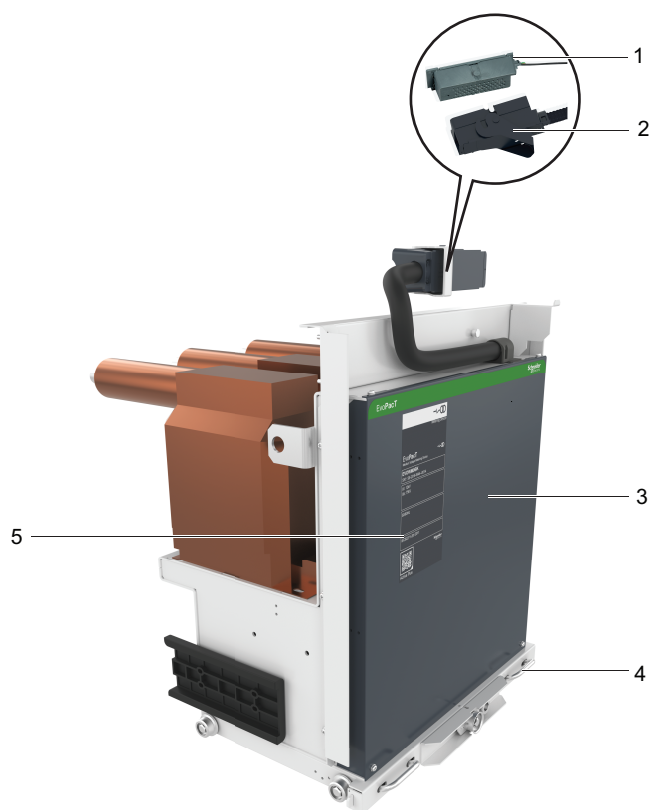
Figure 13 EvoPacT Metering Truck (MTX)
