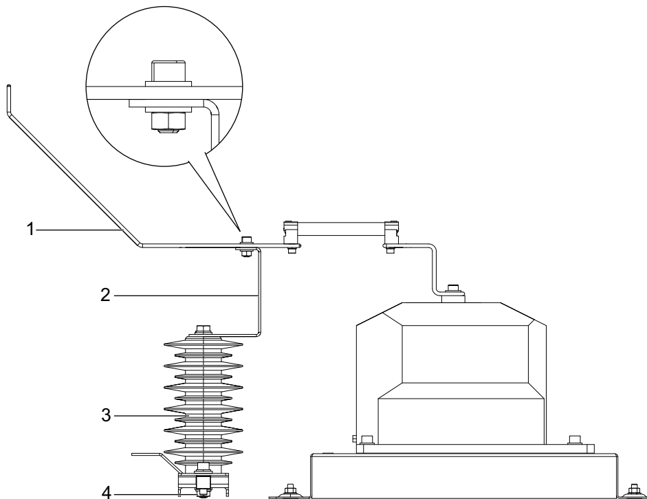
Figure 56 Removal of Surge Arrester Assembly 12/17.5 kV
