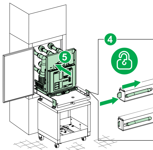
Figure 76 Insertion of VCB into the Cubicle
