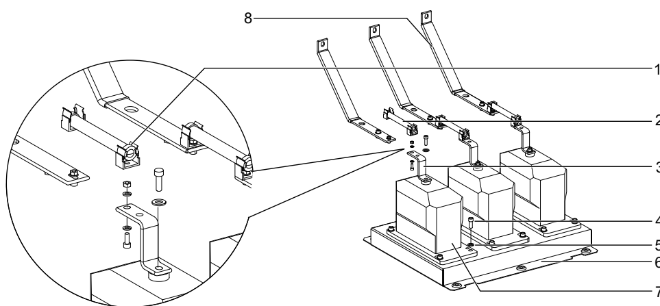
Figure 55 Removal of Fuse and VT 12/17.5 kV
