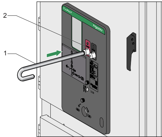
Figure 41 Switching OFF the EvoPacT HVX VCB via Push Rod
