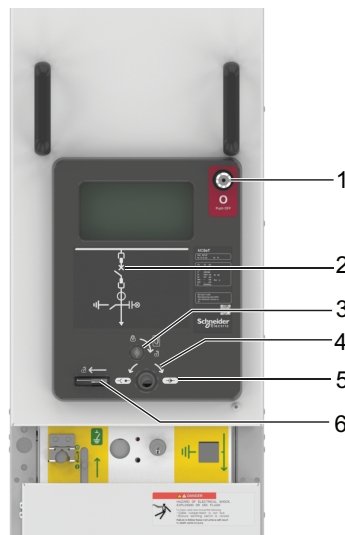
Figure 9 Labels and Indicators on the Feeder with Contactor Cubicle
