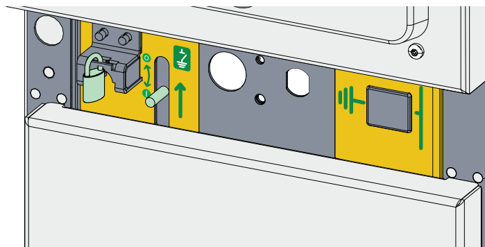
Figure 33 Contactor Cubicle - Mechanical Lock-out of Earthing Switch by Padlock
