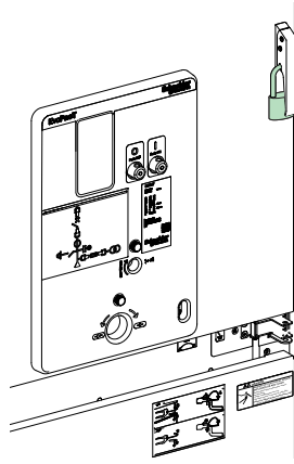
Figure 30 Padlock for the Handle
