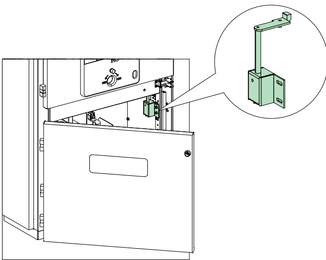
Figure 22 Cable Compartment Door and E/S Interlock, 12/17.5 kV
