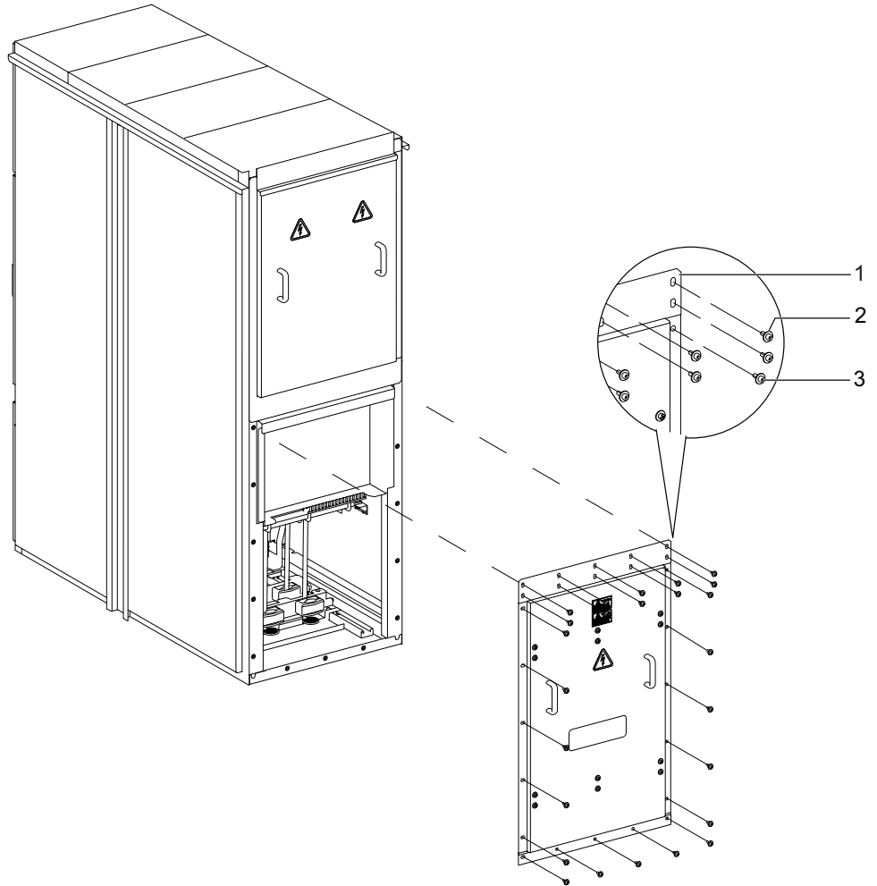
Figure 66 Rear Access of the Cable Compartment 24 kV
