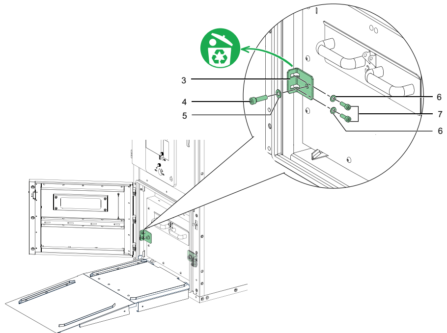
Figure 60 Remove the Transportation Locks
