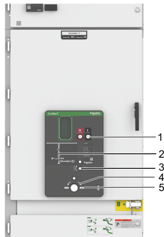
Figure 8 Example of Front View Indicators of I/F Cubicle
