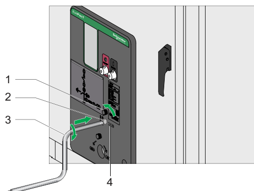
Figure 39 Manual Charging of EvoPacT HVX VCB
