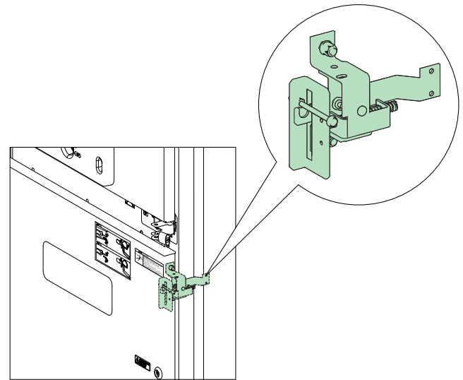
Figure 23 Cable Compartment Door and E/S Interlock, 24 kV
