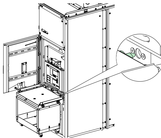
Figure 74 Aligning Trolley with the Cubicle
