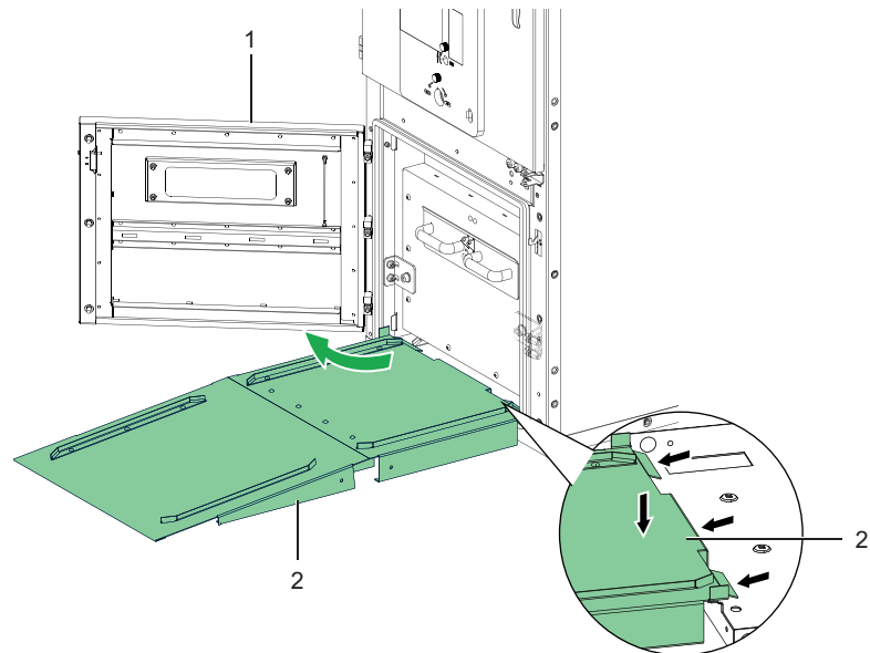
Figure 59 Access to the Withdrawable VT
