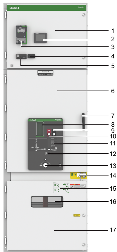
Figure 3 I/F Cubicle
