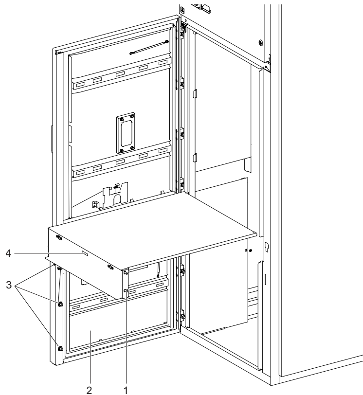
Figure 64 Access to cable compartment via VCB compartment
