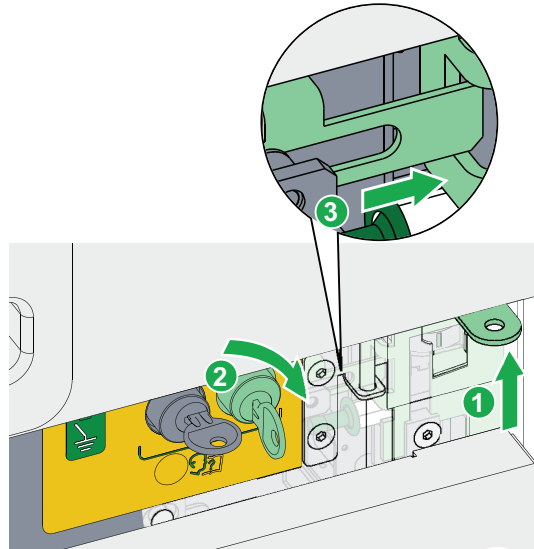
Figure 37 E/S Handle Insertion in OFF Position
