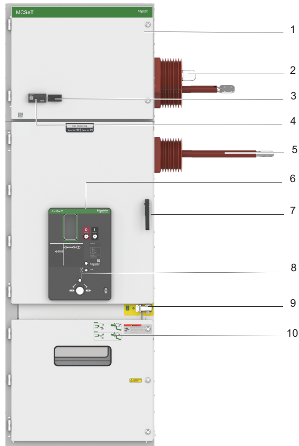
Figure 5 BME Cubicle
