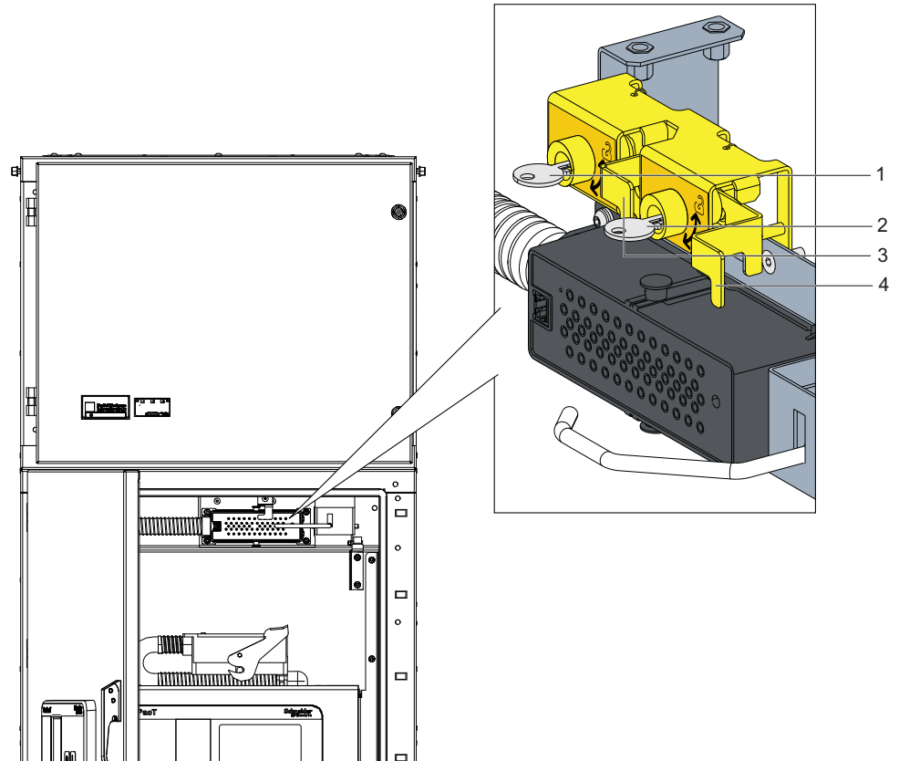
Figure 34 Circuit Breaker Keylocks
