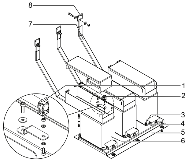
Figure 57 Removal of Fuse and VT 24 kV
