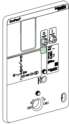
Figure 27 Manual Switching OFF of Circuit Breaker Locked by Padlock
