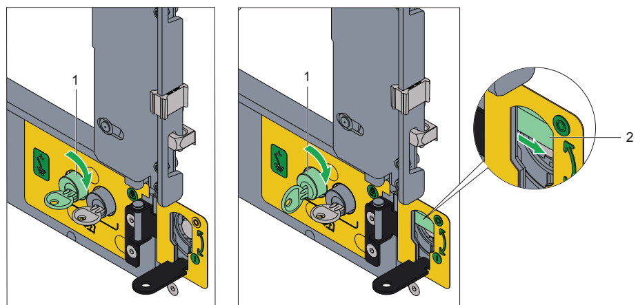
Figure 38 E/S Handle Insertion in ON Position
