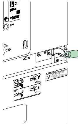
Figure 28 Mechanical Lock-out of Earthing Switch by Padlock
