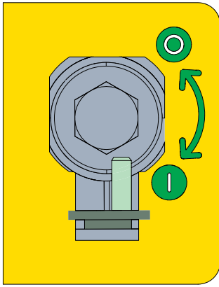
Figure 20 E/S Handle Interlock
