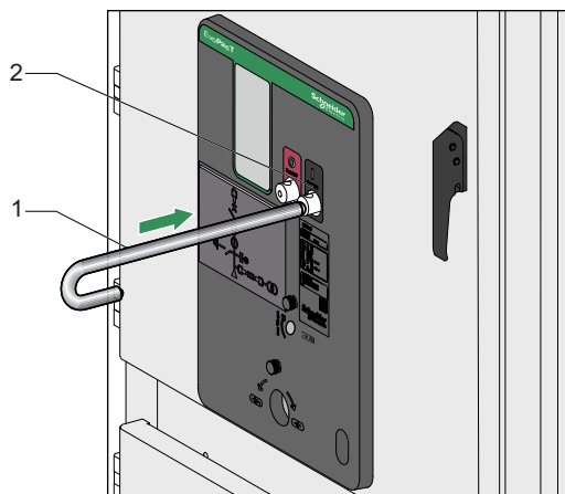
Figure 40 Switching ON the EvoPacT HVX VCB via Push Rod
