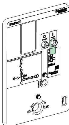
Figure 26 Manual Switching ON of Circuit Breaker Locked by Padlock
