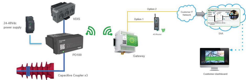
Figure 17 PowerLogic PD100
