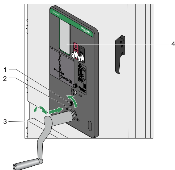
Figure 43 Racking-in the Truck via Truck Handle
