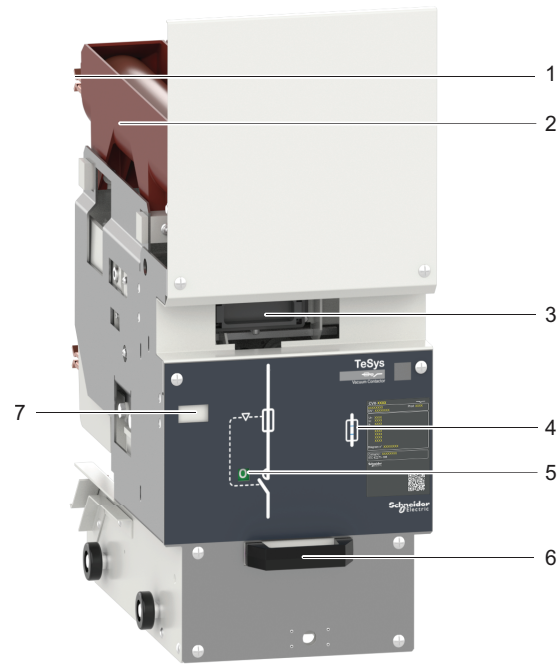
Figure 14 CVX Contactor
