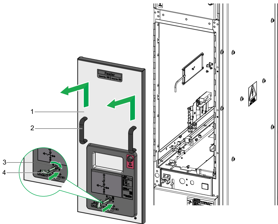
Figure 80 Opening and Closing the Switching Device Compartment Door
