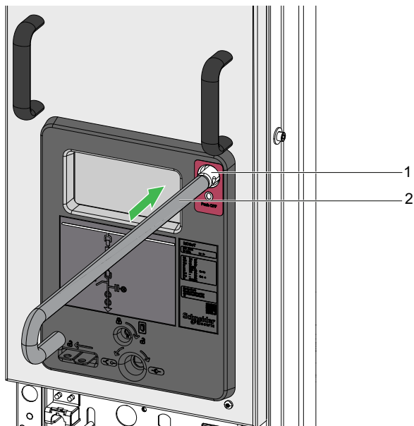
Figure 42 Switching OFF the CVX Contactor via Push Rod
