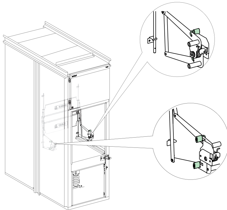
Figure 29 Padlock for the Shutter
