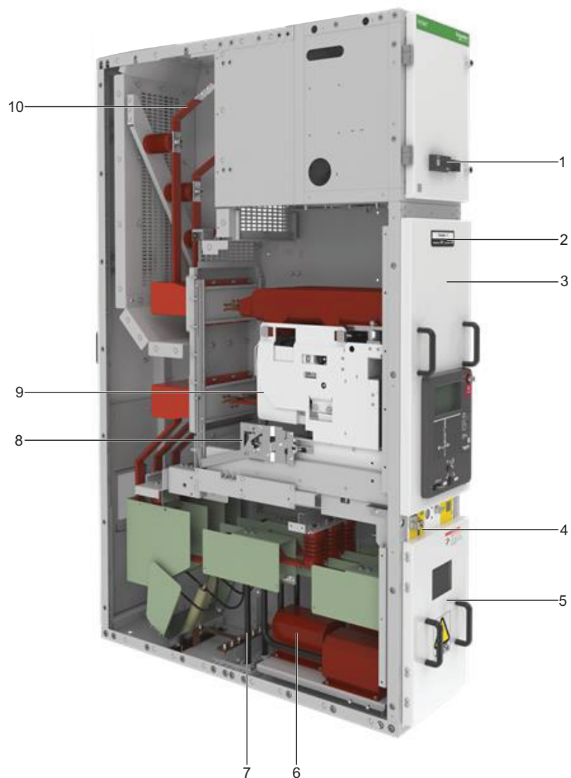
Figure 2 Feeder with Contactor (FC)
