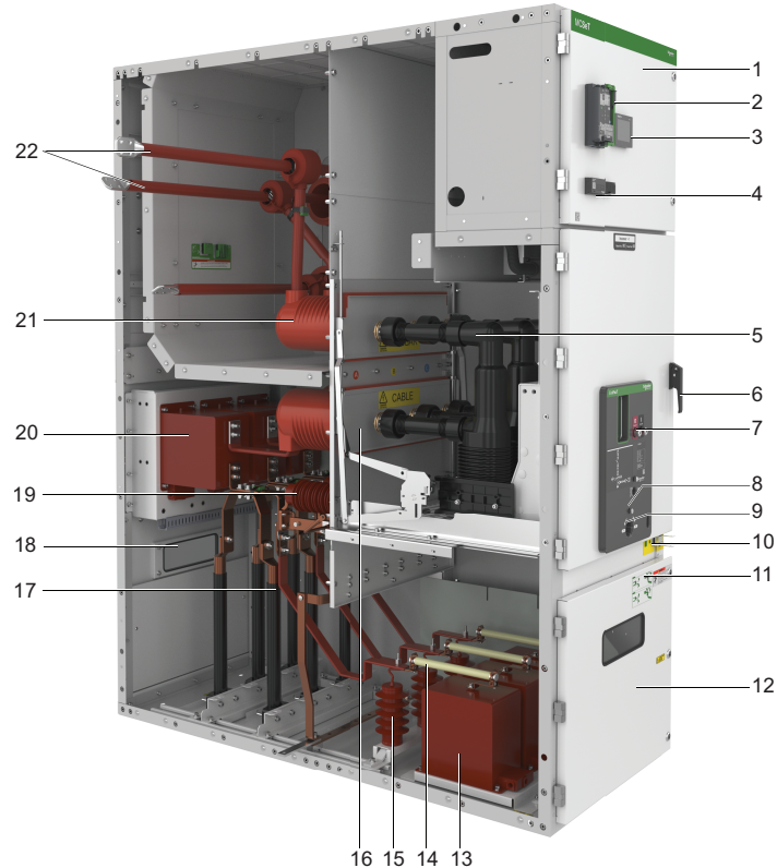
Figure 1 Cubicle Design
