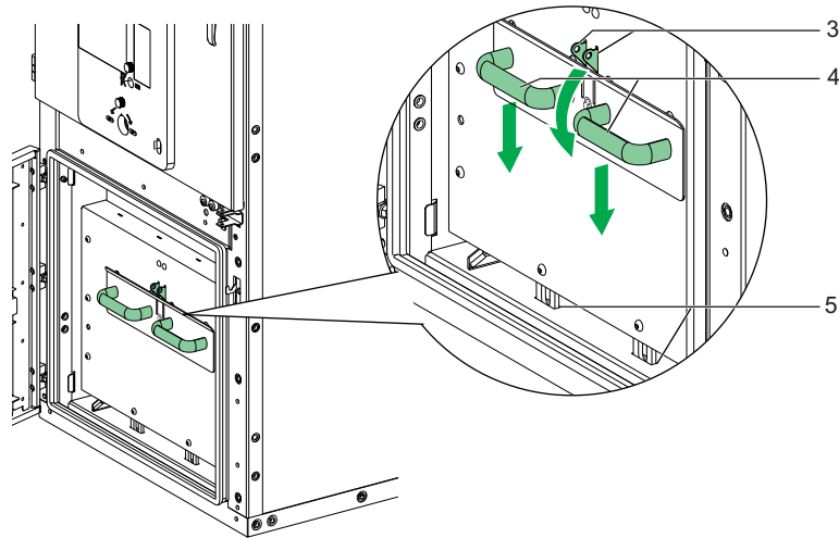
Figure 62 Insertion of withdrawable VT
