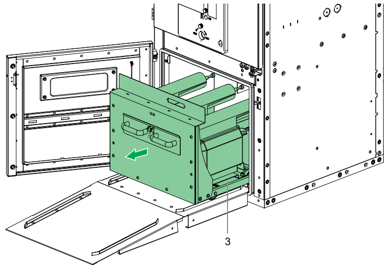
Figure 63 Position the Withdrawable VT
