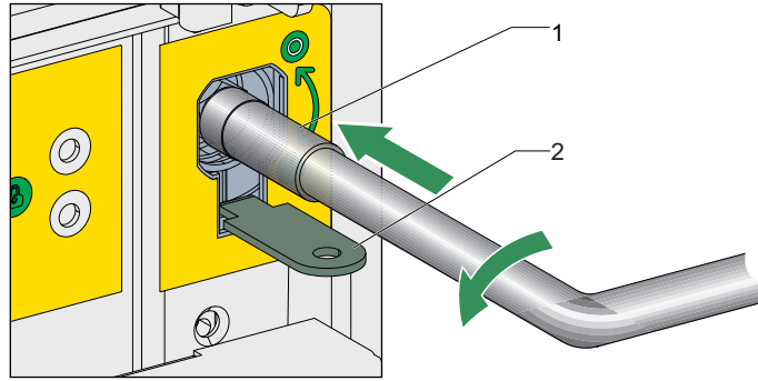
Figure 46 Switching E/S OFF
