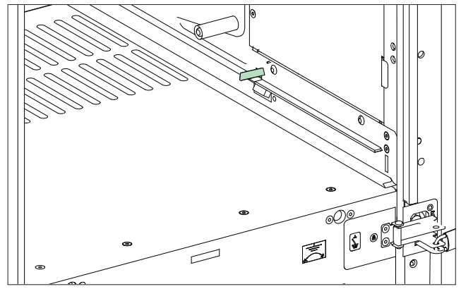
Figure 21 EvoPacT HVX VCB Truck and the E/S Interlock
