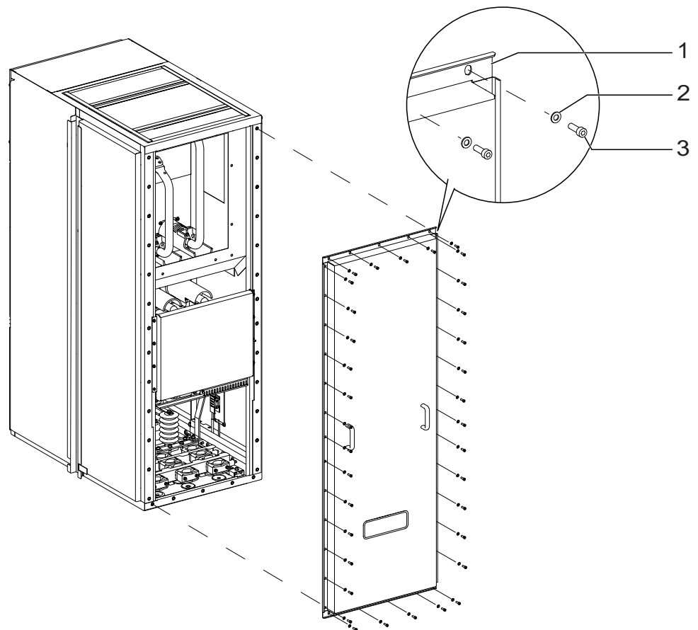
Figure 65 Rear Access of the Cable Compartment 12/17.5 kV
