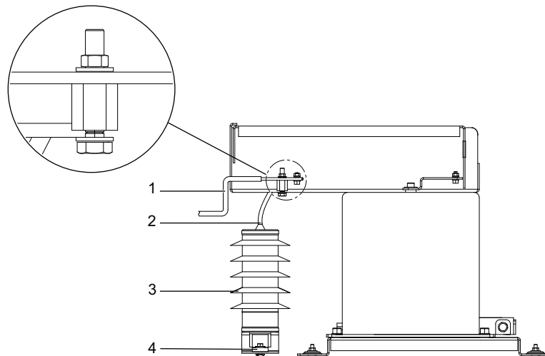
Figure 58 Removal of Surge Arrester Assembly 24 kV
