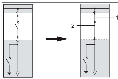
Figure 49 Switch Feeder Cable ON
