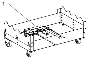
Figure 19 Location of Operation Accessories in the Trolley
