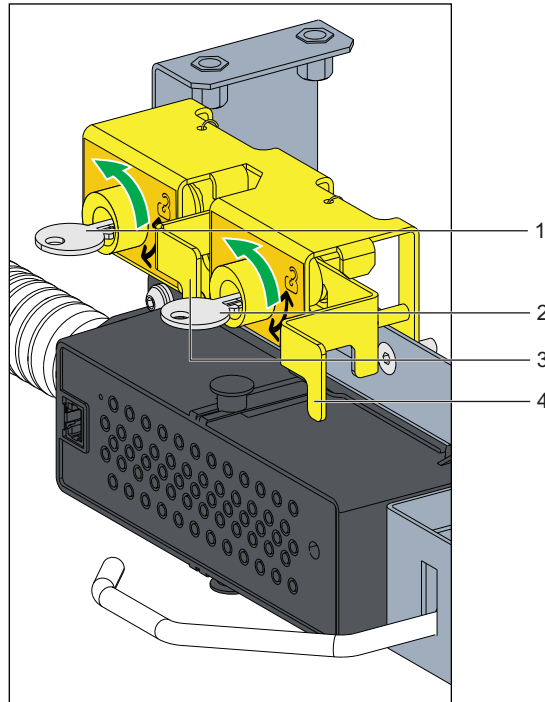
Figure 36 Access to the Circuit Breaker Plug
