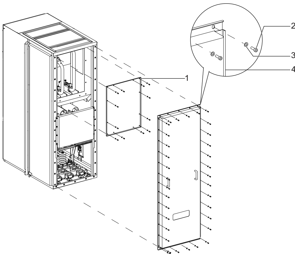
Figure 82 Rear Access of Busbar 12/17.5 kV
