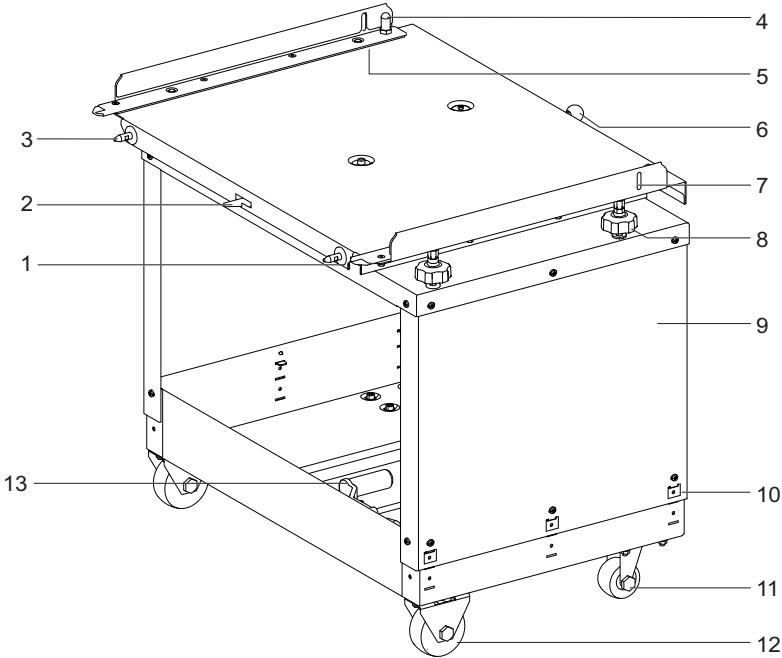
Figure 18 Mechanical Transportation Trolley for the EvoPacT HVX VCB/MTX
