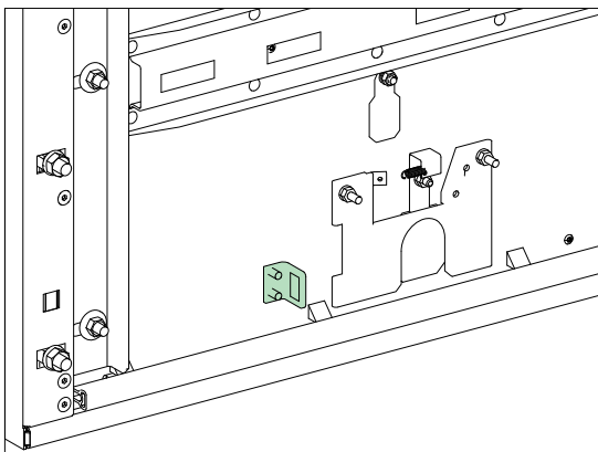
Figure 24 EvoPacT HVX VCB Door and VCB Truck Interlock
