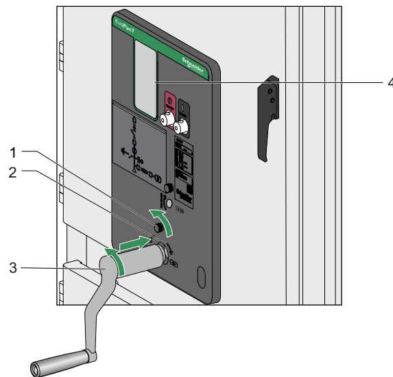
Figure 44 Racking-out the Truck via Truck Handle
