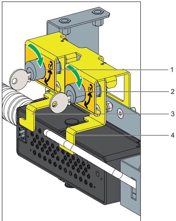
Figure 35 Block the Access to the Circuit Breaker
