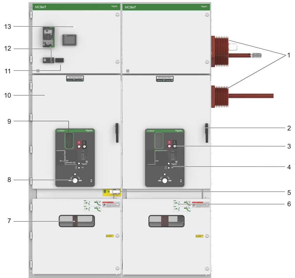
Figure 4 BSC-BSR Cubicles
