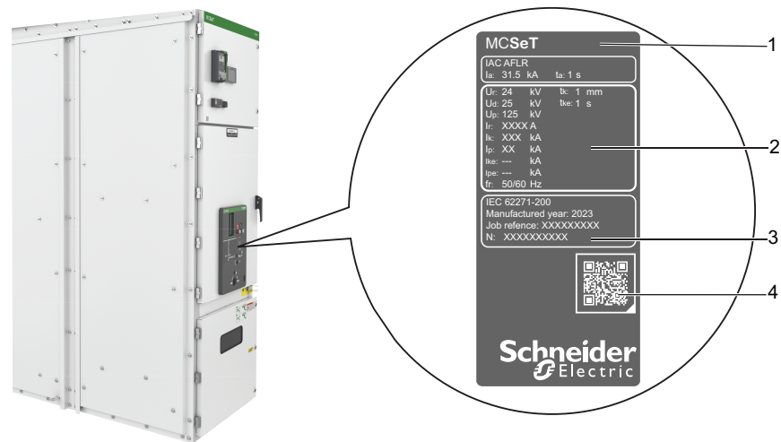
Figure 7 Components of Rating Plate
