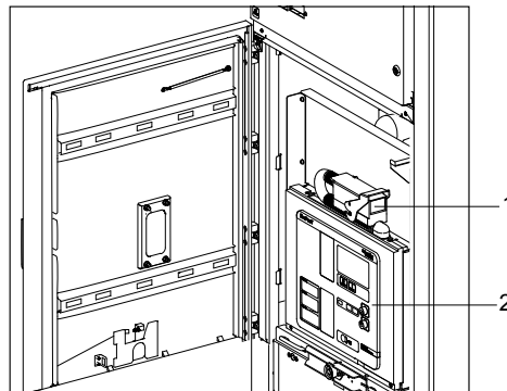
Figure 70 LV Connector Inside the Cubicle
