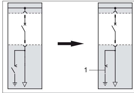
Figure 50 Earthing Feeder Cable
