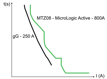
I^2t ON
