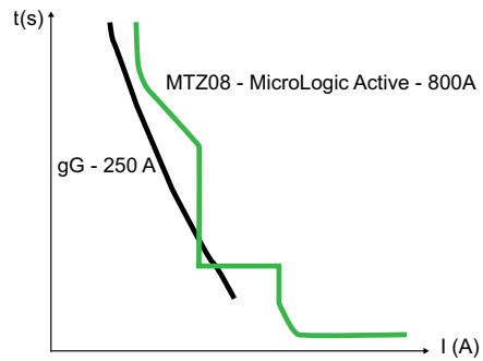
I^2t OFF
