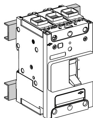
Mounting on rails (Two mounting screws)
